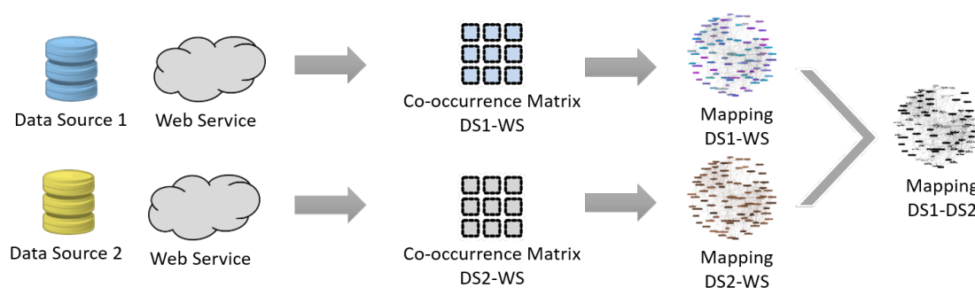
Figure 6. Discovering matching rules between datasets using a web service as a mediator. DS, dataset; WS, web service.
