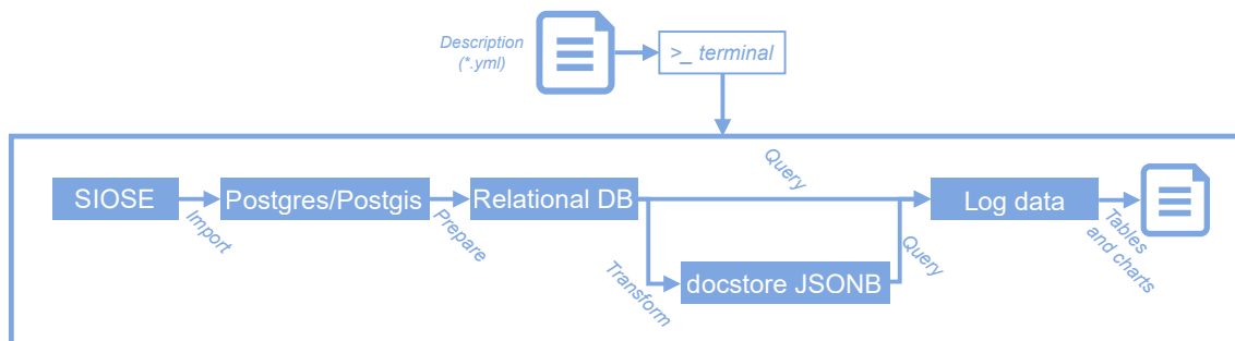
Figure 4. Computational experience in the SIOSE-INNOVA project [23].
