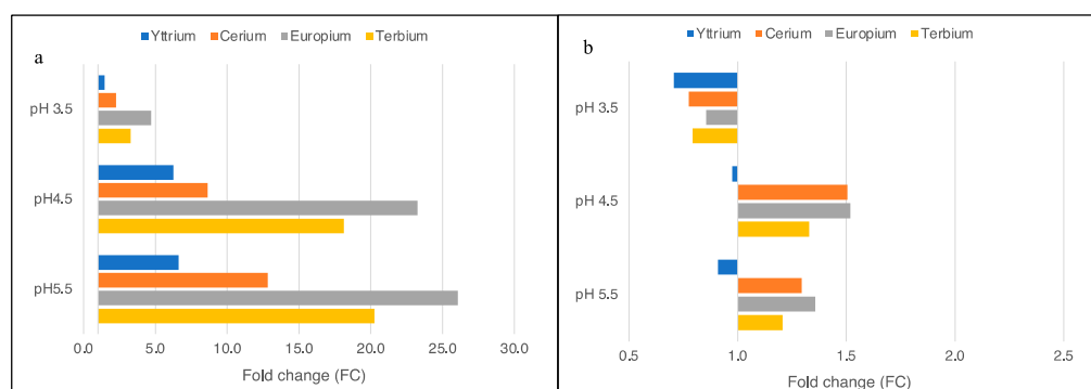
Figure 4. Fold change of the total metal removed from the quaternary-metal aqueous solutions by G. sulphuraria , strains SAG 107.79 (a) and ACUF 427 (b). The fold change was calculated by comparing the \mu\text{mol/g dm} of every metal obtained at pH 3.5, 4.5, and 5.5 with the \mu\text{mol/g dm} measured at pH 2.5.
