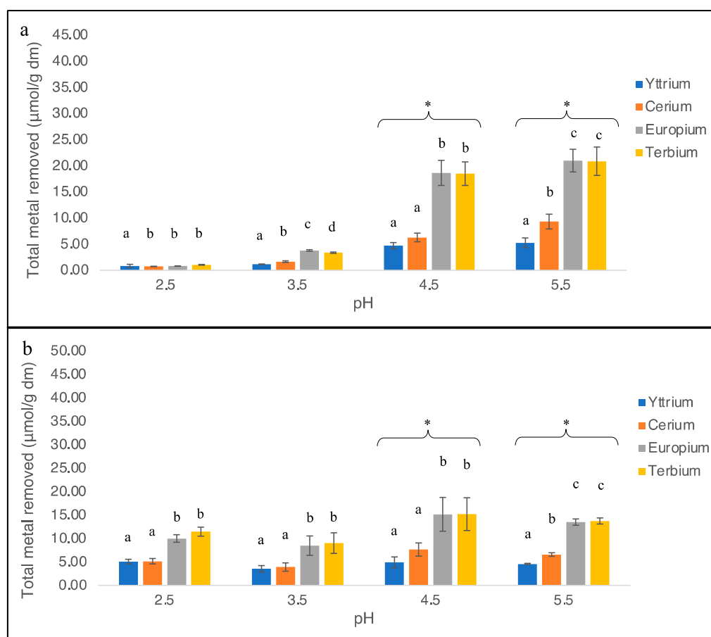
Figure 3. The metal removed from the quaternary-metal aqueous solutions by G. sulphuraria , strains SAG 107.79 (a) and ACUF 427 (b). Data were divided based on the pH of the solutions. Different letters in the same experiment indicate a significant difference, p < 0.05 ; Symbol (*) indicates a p < 0.05 significant difference compared to the pH 2.5.
