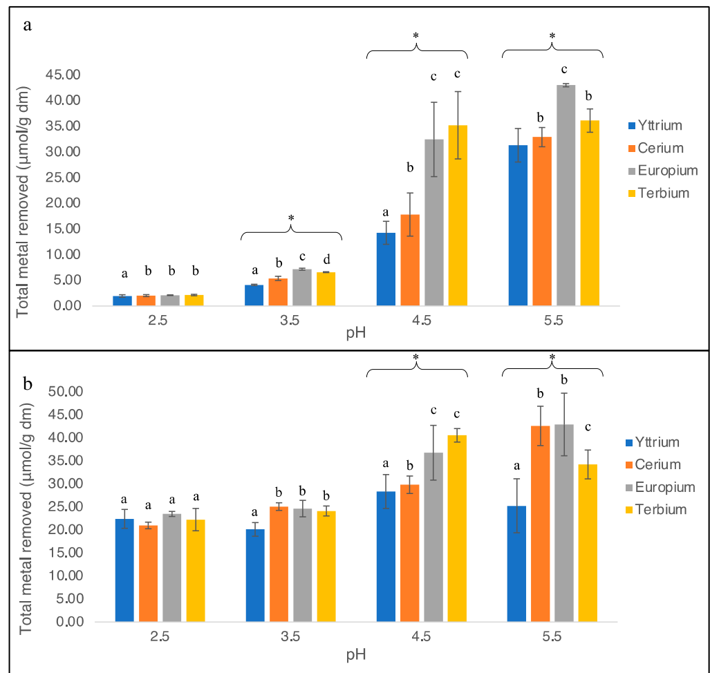
Figure 1. Metal removed from the single-metal aqueous solutions by G. sulphuraria , strains SAG 107.79 (a) and ACUF 427 (b). Data were divided based on the pH of the solutions. Different letters in the same experiment indicate a significant difference, p < 0.05 ; Symbol (*) indicates a p < 0.05 significant difference compared to the pH 2.5.
