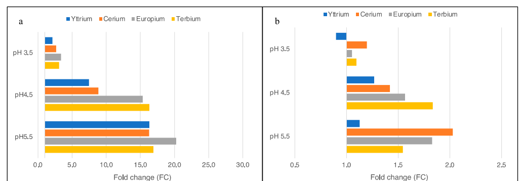
Figure 2. Fold change of the total metal removed from the single-metal aqueous solutions by G. sulphuraria , strains SAG 107.79 (a) and ACUF 427 (b). The fold change was calculated by comparing the \mu\text{mol/g dm} of every metal obtained at pH 3.5, 4.5, and 5.5 with the \mu\text{mol/g dm} measured at pH 2.5.
