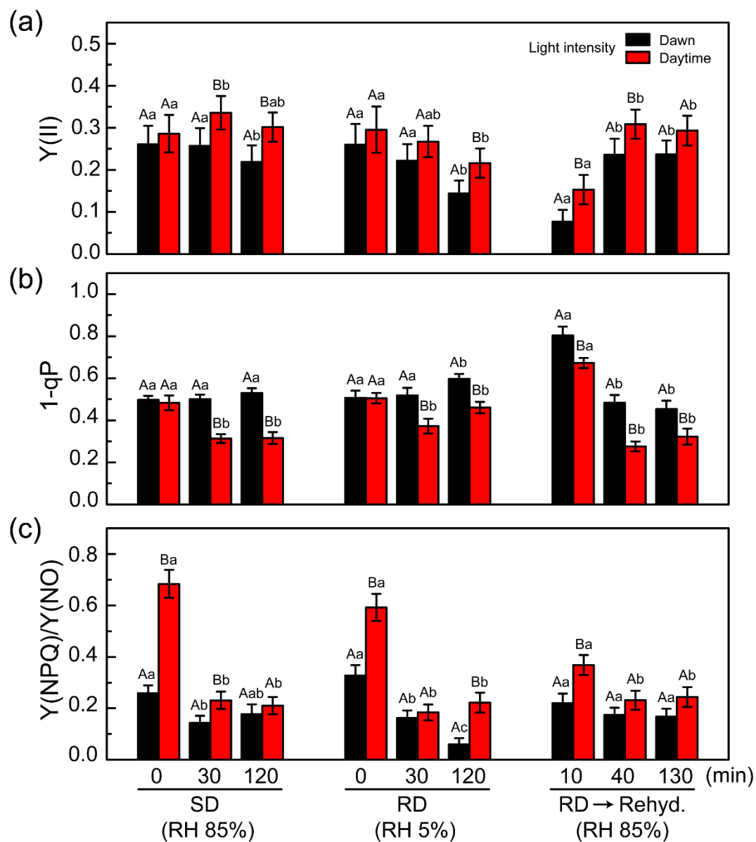
Figure 5. PSII photochemistry changes during RLC experiments under the given conditions. (a) Effective photosynthetic yield Y(II), (b) 1-qP value, and (c) Y(NPQ)/Y(NO) ratio. Each value indicates the average score \pm standard deviation, calculated from the data in Figure S6. The average was calculated by two-way ANOVA, and its significant differences among the data were analyzed based on the Tukey's HSD test (at p < 0.05 ) which was displayed with different letters; upper case letters indicate the effects of light intensity at the same time of desiccation (or rehydration) treatment, and lower case letters indicate the effects of desiccation (or rehydration) treatment at the same light condition. The ten biological replicates were used for each treatment ( n = 10 ). Experiments were repeated at least two or three times using the same thalli after re-stabilizing at 50 \mu\text{mol}/\text{m}^2/\text{s} light with an 18:6 light:dark cycle at 8^\circ\text{C} with hydration for a week. Black and red bars represent dawn light ( 50 \mu\text{mol}/\text{m}^2/\text{s} ) and daylight ( 220 \mu\text{mol}/\text{m}^2/\text{s} ), respectively. Y(NPQ), the efficiency of the regulated non-photochemical quenching reaction; Y(NO), the efficiency of the nonregulated non-photochemical quenching reaction; SD, slow desiccation; RD, rapid desiccation; RD→Rehyd., rehydration after 24 h of RD treatment.
