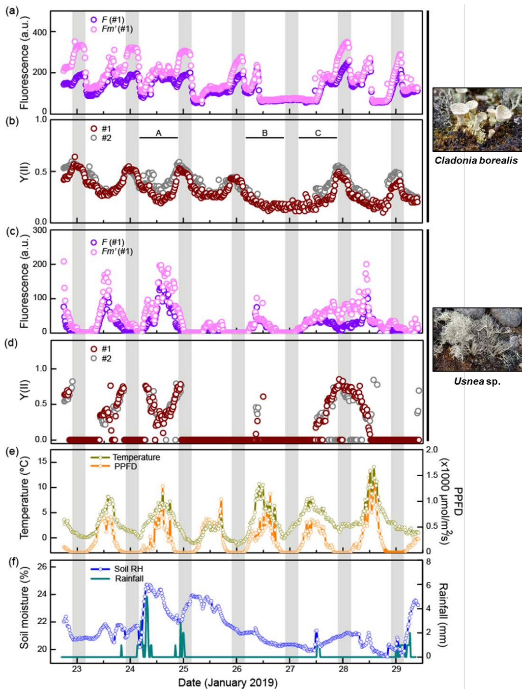
Figure 2. Field observation of the fluorescence ( F and Fm' ) and Y(II) value of C. borealis and Usnea sp. and microclimate at the site. Grey shading indicates nighttime (10 PM to 4 AM) when photosynthetic photon flux density (PPFD) was less than 10 \mu\text{mol}/\text{m}^2/\text{s} . (a,b) Fluorescence and Y(II) value of C. borealis (c,d) Fluorescence and Y(II) value of Usnea sp. Data were obtained from two individual thalli (Samples #1, #2). Patterns of fluorescence ( F and Fm' ) of C. borealis and Usnea sp. were similar between the two samples. (e) Changes in temperature ( ^{\circ}\text{C} ) and PPFD ( \mu\text{mol}/\text{m}^2/\text{s} ). (f) Changes in volumetric soil moisture (%) and rainfall (mm) during the observation period. F , current fluorescence; Fm' , maximum fluorescence.
