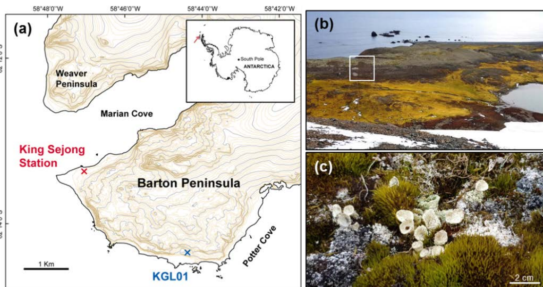
Figure 1. Location and landscape of the study site (KGL01: 62°14'24" S, 58°44'36" W), and an image of C. borealis at the field. (a) KGL01 on the map, placed near Potter Cove in Barton Peninsula. (b) This site has well-distinguished vegetation that consists of mosses and lichens. The area spanning the brown and grey parts was composed of lichens, and our observation was performed at the area indicated by the white box. (c) Several thalli of C. borealis accompanied by the moss Chorisodontium aciphyllum are shown.
