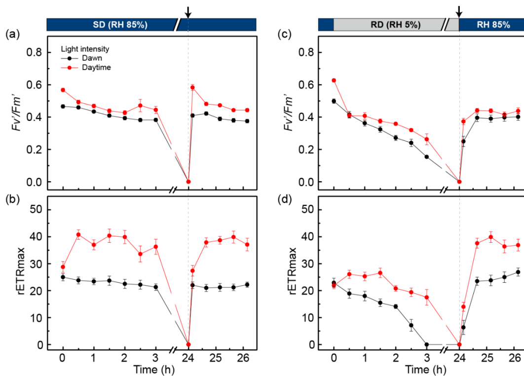
Figure 4. Changes in maximal photosynthetic yield ( F_v'/F_m' ) (a,c) and rETRmax (b,d) with dawn-light (50 \mu\text{mol}/\text{m}^2/\text{s} ) and daytime-light (220 \mu\text{mol}/\text{m}^2/\text{s} ) under a desiccation-rehydration cycle in C. borealis . Before desiccation, samples were activated with light (50 \mu\text{mol}/\text{m}^2/\text{s} ) for 2 h under fully hydrated conditions with distilled water. The thalli were treated under slow desiccation (SD, 85% RH) (a,b) and rapid desiccation (RD, 5% RH) (c,d) for 24 h (until indicated by the dashed line), and then rehydrated with a water spray of distilled water (black arrow). After the removal of excess water, both samples were kept under SD conditions for an additional 2 h. The ten biological replicates were used for each treatment ( n = 10 ). Experiments were repeated at least two or three times using the same thalli after re-stabilizing at 50 \mu\text{mol}/\text{m}^2/\text{s} light with an 18:6 light:dark cycle at 8 °C with hydration for a week. Results are the means with \pm standard deviation shown by vertical bars.
