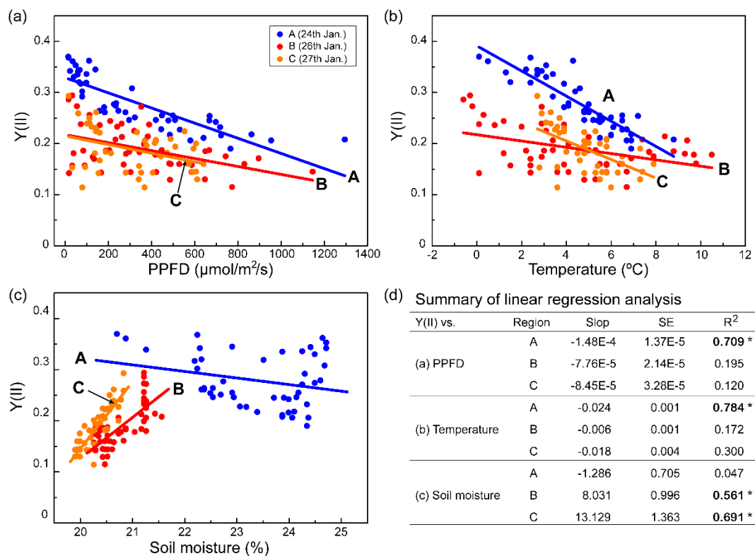
Figure 3. Correlation between Y(II) of C. borealis and PPFD (a), temperature (b), and volumetric soil moisture (c) parameters. Data were extracted from Regions A, B, and C in Figure 2b. A fitting analysis for linear regression was performed for each dataset. (d) The linear regression parameters are presented in a tabular format. Asterisks indicate R^2 > 0.5 . SE, standard error.
