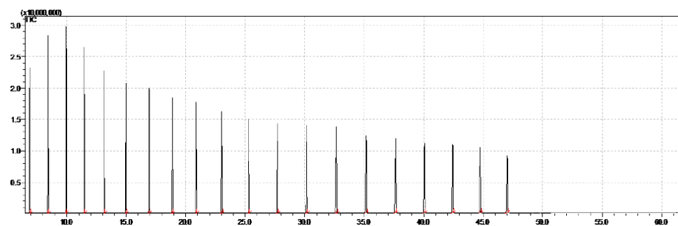
Figure S2. GC-MS chromatograms of n-alkane standard.
