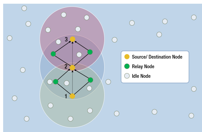
Figure 5. Data transmission in Cooperative Depth Based Routing (CoDBR) [54].
