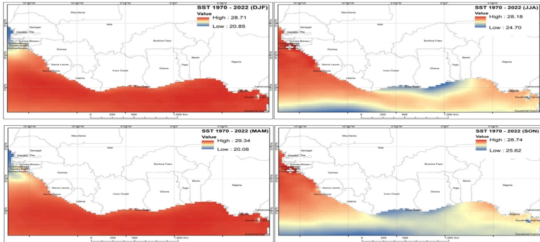
Figure 2. Seasonal patterns of SST variability.
