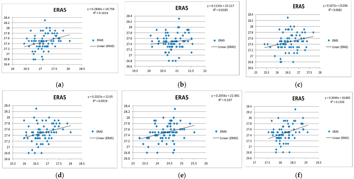
Figure 12. Evaluation of CMIP6 model’s performance against ERA5 regression analysis: (e) Figure 10: Evaluation of CMIP6: (a) ACCESS, (b) CAMS-CSM, (c) CAN-ESM, (d) CMCC-MCM-UA, and (f) MPI-ESM models.
