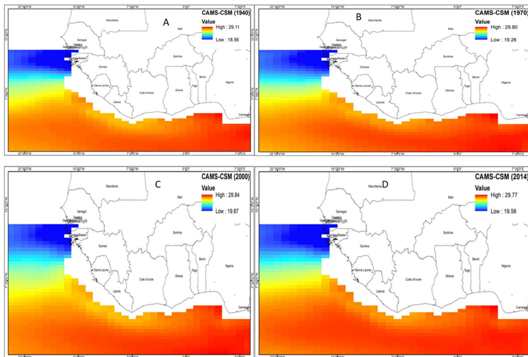
Figure 4. CMIP6 CAMS-CSM model's historical simulation.
