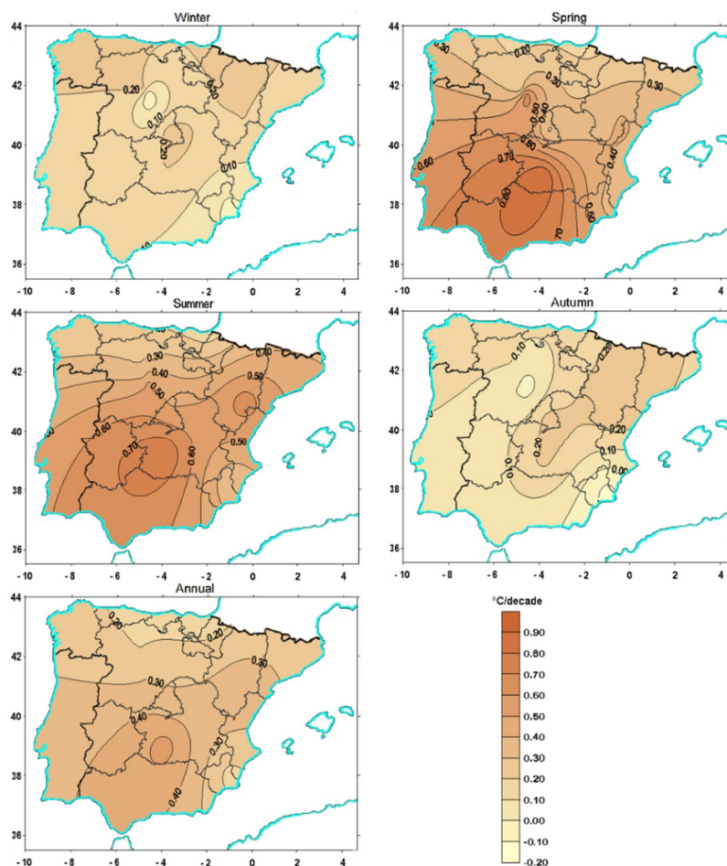
Figure 3. Isolines of seasonal and annual trends in maximum temperature anomalies in Spain over the period 1950–2011, expressed in °C decade -1 .
