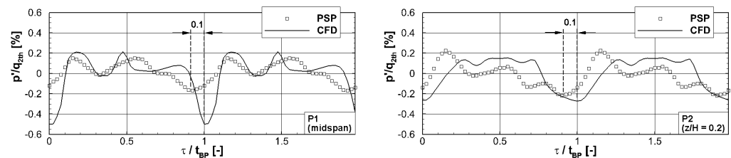
Figure 12. Comparison of CFD predictions of pressure fluctuations to phase-locked PSP measurements at position P1 (left) & P2 (right) marked in Figure 9.
