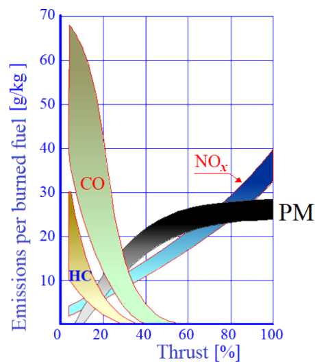
Figure 9. Emissions vs. thrust.
