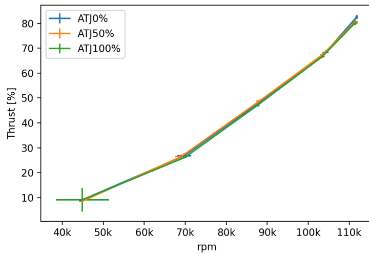
Figure 11. GTM-140/ATJ: Thrust.
