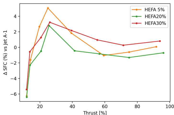
Figure A2. DGEN 380/HEFA: SFC changes.
