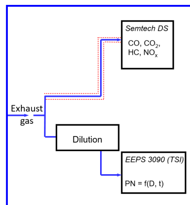
Figure 6. Exhaust gas sampling.
