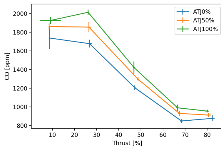
Figure 13. GTM-140/ATJ: CO emission.
