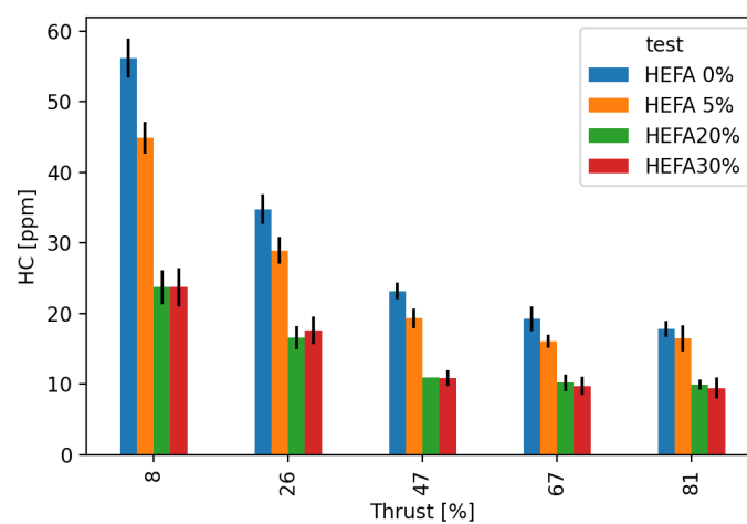
Figure 22. GTM-140/HEFA: HC emission.
