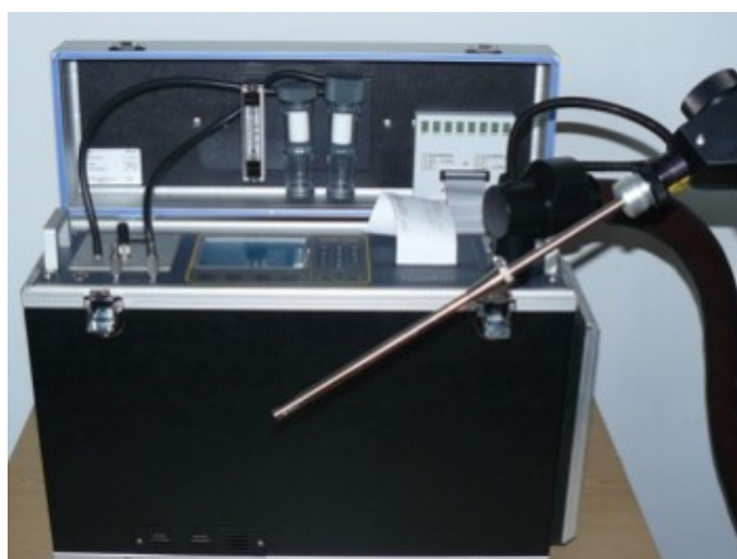
Figure 3. GA-60 emissions analyser.
