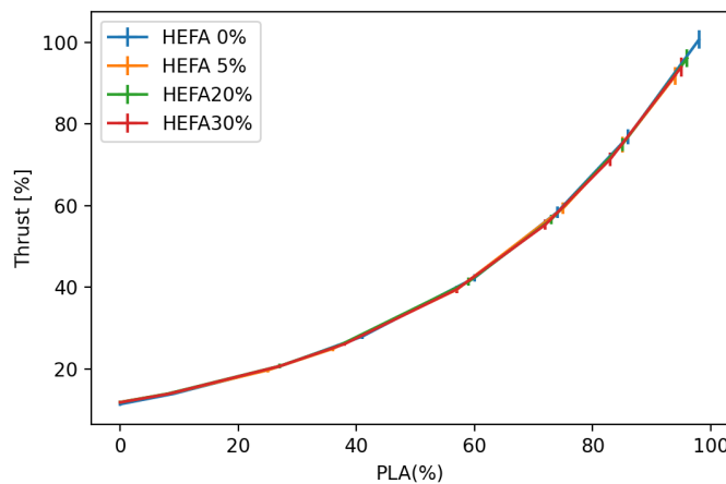
Figure 24. DGEN 380/HEFA: Thrust vs. PLA.
