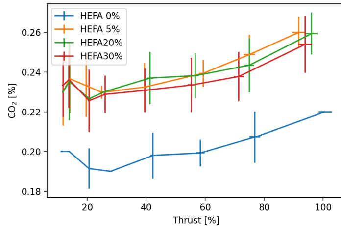
Figure 32. DGEN 380/HEFA: CO 2 .
