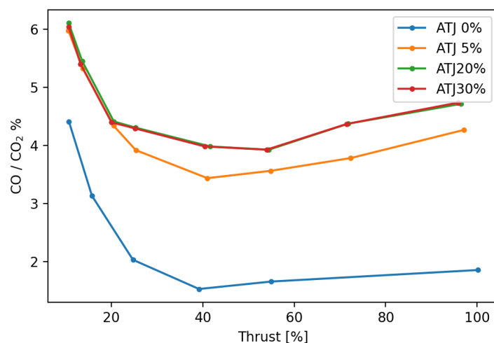
Figure 33. DGEN 380/ATJ: CO vs. CO 2 .
