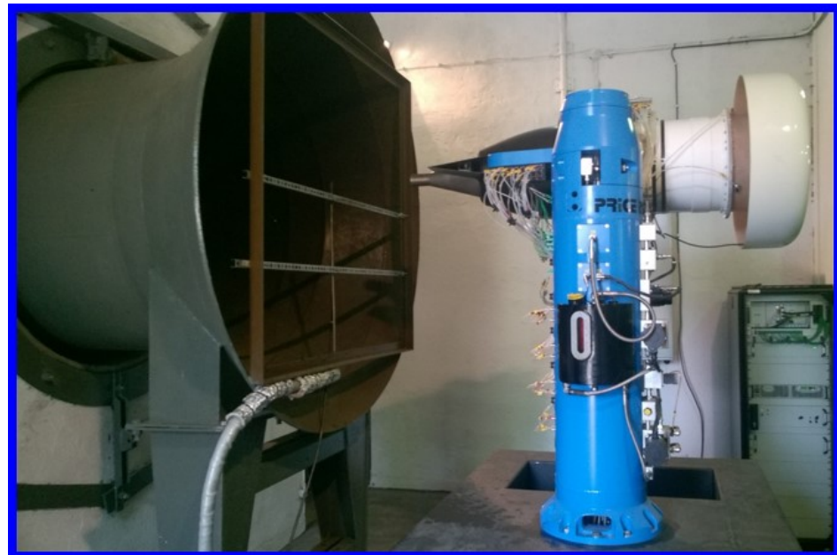
Figure 8. Test cell.
