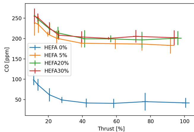
Figure 31. DGEN 380/HEFA: CO.
