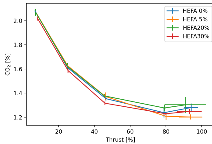
Figure 20. GTM-140/HEFA: CO 2 emission.
