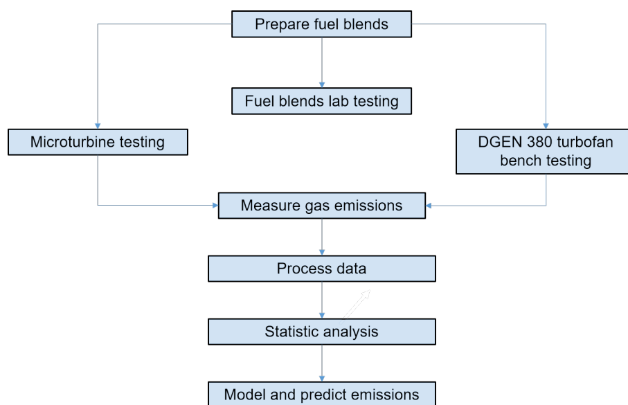
Figure 1. Testing methodology.
