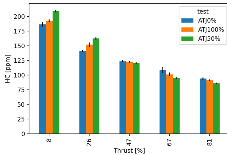
Figure 15. GTM-140/ATJ: HC emission.
