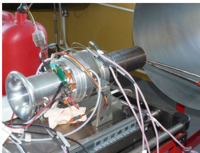
Figure 2. GTM-140 microturbine.
