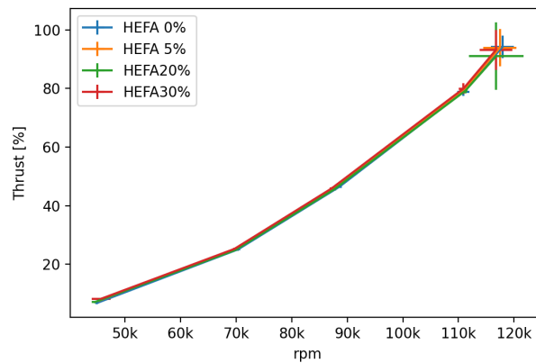
Figure 17. GTM-140/HEFA: Thrust.
