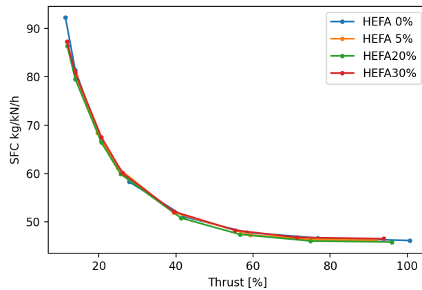
Figure 26. DGEN 380/HEFA: SFC.
