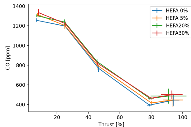
Figure 19. GTM-140/HEFA: CO emission.
