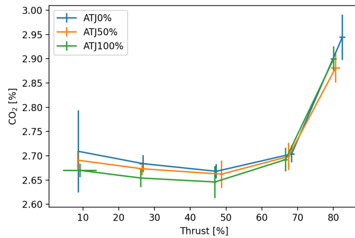
Figure 14. GTM-140/ATJ: CO 2 emission.
