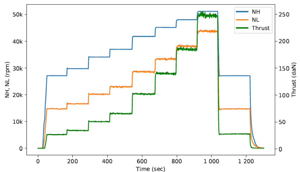
Figure 10. Engine test profile for DGEN 380.
