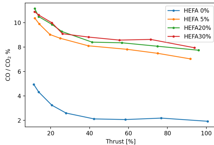
Figure 34. DGEN 380/HEFA: CO vs. CO 2 .
