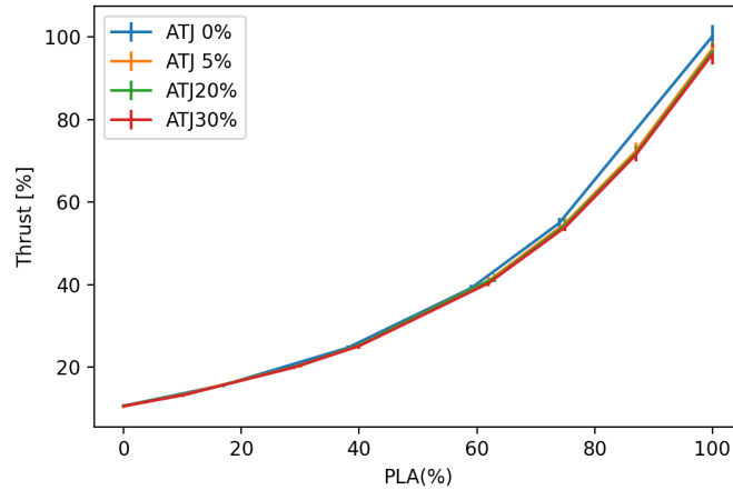
Figure 23. DGEN 380/ATJ: Thrust vs. PLA.
