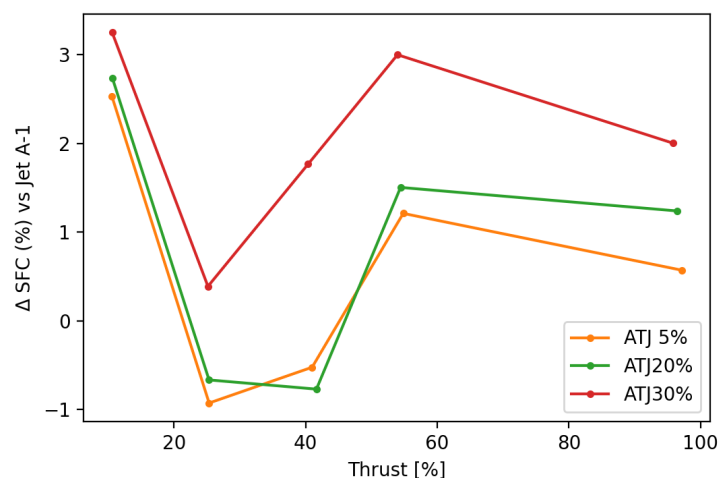
Figure A1. DGEN 380/ATJ: SFC changes.
