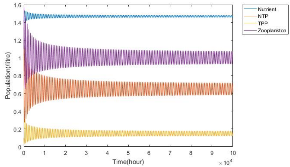
Figure 10. Simulation results of System (2) with \tau < \tau_0 .
