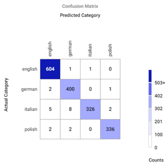
Figure A13. Classification error matrix among accents set EN, GE, IT, PO .
