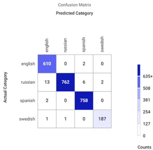
Figure A12. Classification error matrix among accents set EN, RU, SP, SW .
