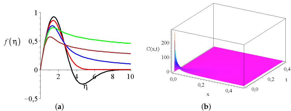
Figure 5. (a) Functions of Equation (45) for \alpha = 1 where black, red, blue, green and brown lines are for \beta = 1/4, 1/2, 1, 2 and 3 , (b) The C(x, t) solution of Equation (46) for \alpha = \beta = 1 .
