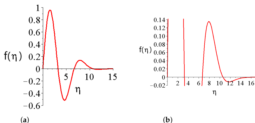
Figure 6. (a) Functions of Equation (45) for \alpha = 1 when \beta = 1/8 , (b) magnification of f(\eta) for values close to zero.
