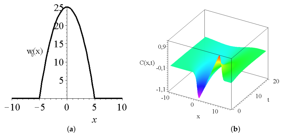
Figure 3. (a) The initial condition of Equation (15), (b) the full solution C(x, t) of Equation (16).
