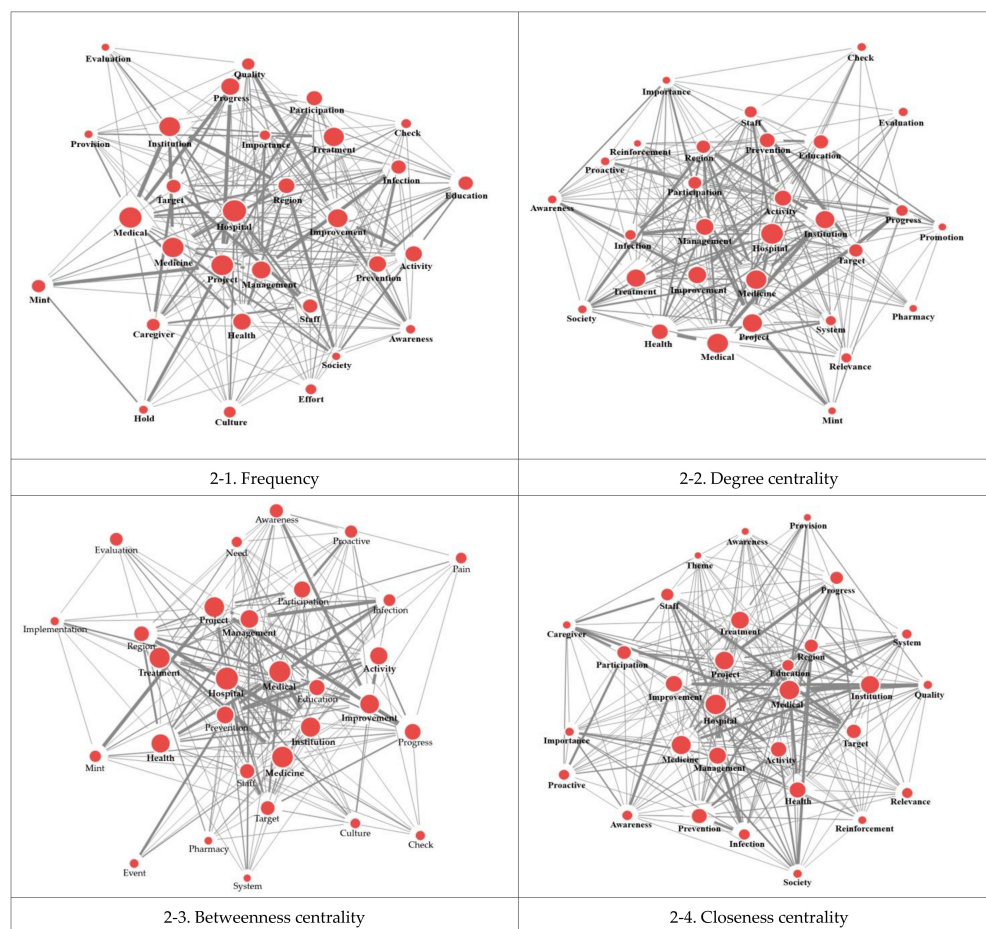
Figure 2. Spring network map of centrality.
