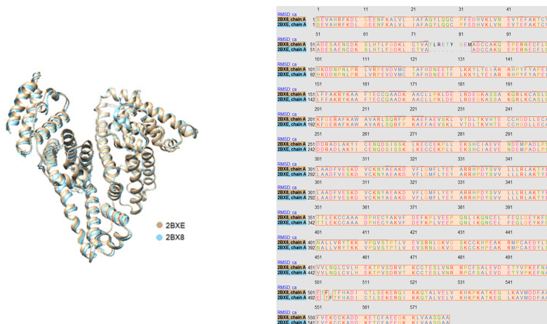
Figure 5. Overlay of PDB 2BX8 and PDB 2BXE structures performed in Chimera 1.15 software and representation of the sequence of the amino acid alignment of the structures.
