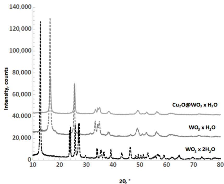
Figure 5. XRD diagrams of WO 3 ·2H 2 O NLS, WO 3 ·H 2 O NLS, and Cu 2 O@WO 3 ·H 2 O nanocomposite (0.5 molar equivalent CuMes/W atom).
