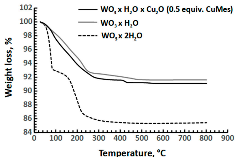
Figure 6. TGA analysis of WO 3 ·2H 2 O NLS, WO 3 ·H 2 O NLS, and Cu 2 O@WO 3 ·H 2 O nanocomposite (0.5 molar equivalent CuMes/W).
