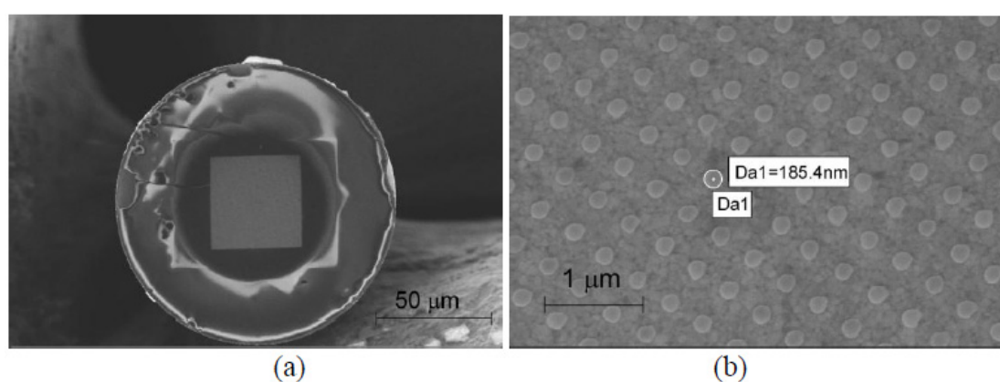
Figure 25. SEM images of a gold nanodot array on an optical fiber tip: (a) Overview of the optical fiber end facet; (b) Gold nanodot array on the optical fiber facet. Reprinted with permission of [89].
