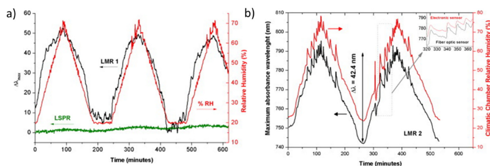
Figure 11. Evolution of the dynamic response of the optical fiber sensors composed of 25 bilayers (a) and 40 bilayers (b), respectively. Reprinted with permission of [52].
