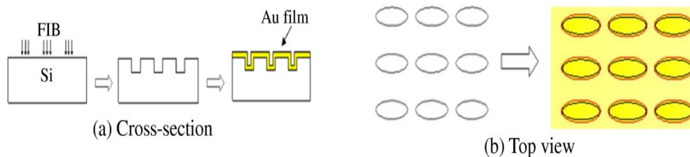
Figure 28. Schematic images of the process of Focused Ion Beam (FIB) pre-milling with the following thermal evaporation: (a) Cross section of the nanostructures before and after thermal evaporation; (b) top view of the nanostructures. Reprinted with permission of [94].
