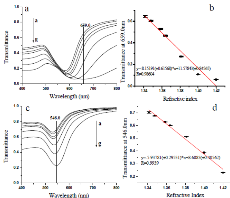
Figure 20. (a) and (c) Transmission spectra at variable sucrose concentrations by using the 48-nm and 23-nm Au NP films; (b) Transmission at 659.07 nm of 48-nm AuNPs as a function of the refractive index value; (d) Transmission at 546.0 nm of 23-nm AuNPs as a function of the refractive index value. Reprinted with permission of [73].
