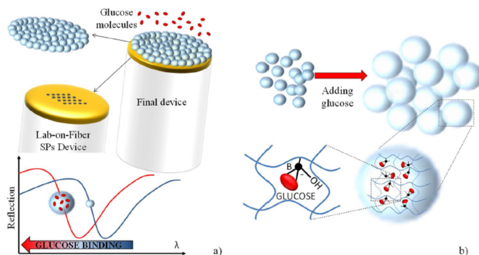
Figure 35. (a) Schematic of the developed device based on the combination of microgels (MGs) and LOF Technology; (b) Schematic view of the glucose-binding event inside the MGs network. Reprinted with permission of [97].
