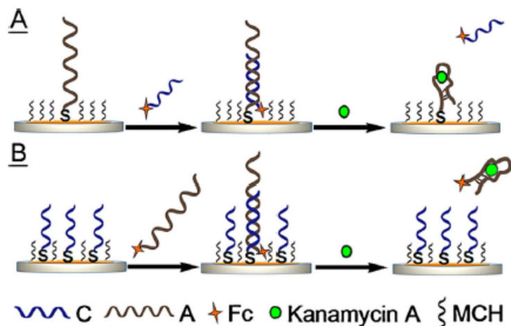
Figure 11. Schematic illustration of two approaches for the development of an electrochemical aptasensor for the detection of kanamycin A based on signaling-probe displacement. Reprinted from reference [40], with permission from Elsevier.
