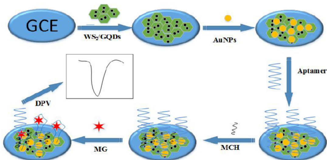
Figure 6. Working principle of a label free electrochemical aptasensor for the detection of malachite green. Reprinted from reference [31]. This article is an open access article distributed under the terms and conditions of the Creative Commons Attribution (CC BY) license ( http://creativecommons.org/licenses/by/4.0/ 25 March 2021).
