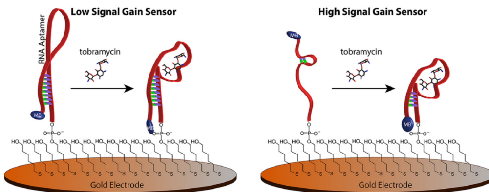
Figure 4. Schematic illustration of two electrochemical aptasensor architectures: a low signal gain sensor and a high signal gain sensor. The latter illustration shows a larger change in conformation upon target binding thus leading to a high signal change. Reprinted with permission from Schoukroun-Barnes LR, Wagan S, White RJ. 2014. Enhancing the Analytical Performance of Electrochemical RNA Aptamer-Based Sensors for Sensitive Detection of Aminoglycoside Antibiotics. Anal. Chem. 86:1131–1137. Copyright (2013) American Chemical Society.
