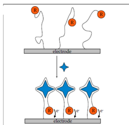
Figure 5. Working principle of a labelled electrochemical aptasensor based on target induced conformation change. The aptamer was previously labelled with a redox probe on its free extremity. The aptamer conformation was modified in the presence of the target analyte (a) the distance between the redox probe to the electrode surface was decreased (“signal on”). Reprinted from reference [16]. This article is an open access article distributed under the terms and conditions of the Creative Commons Attribution (CC BY) license ( http://creativecommons.org/licenses/by/4.0/ 25 March 2021).
