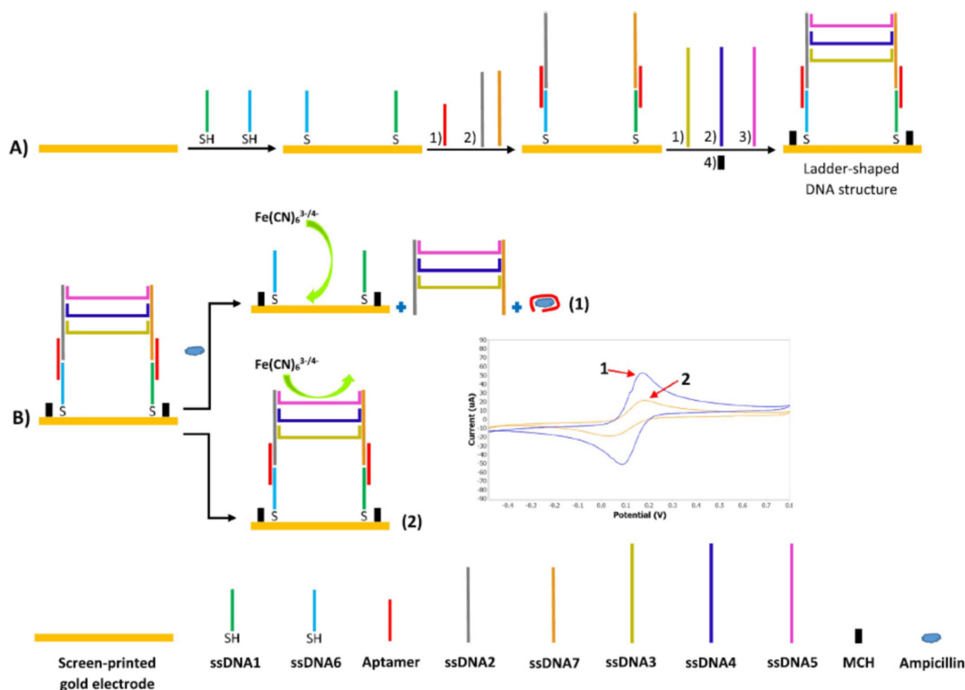
Figure 7. Schematic illustration of a label-free electrochemical aptasensor based on ladder-shaped DNA structure for the detection of ampicillin in milk. Reprinted from reference [32] with permission from Elsevier.
