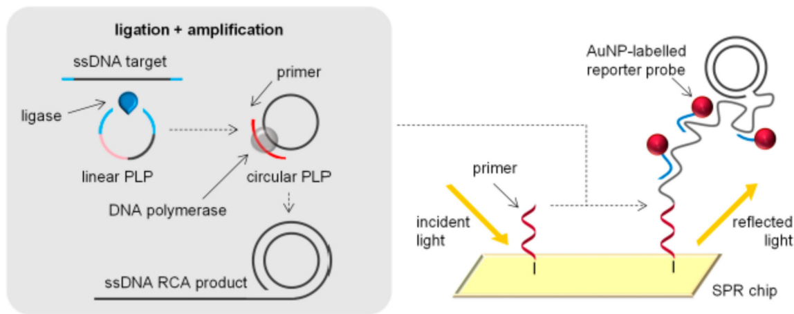
Figure 23. Schematic illustration of an optical aptasensor based on Rolling circle amplification (RCA). Reprinted from [141]. This article is an open access article distributed under the terms and conditions of the Creative Commons Attribution (CC BY) license ( https://creativecommons.org/licenses/by/4.0/ 25 March 2021)).
