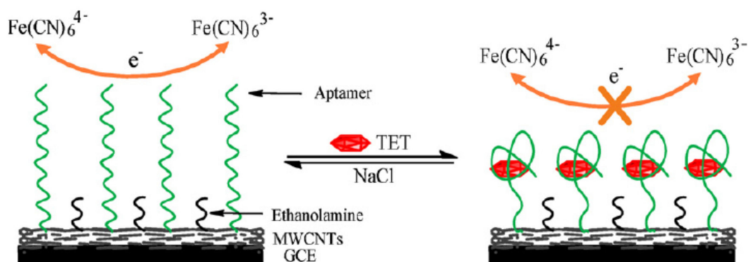
Figure 13. Fabrication of aptasensors modified with multi-walled carbon nanotubes (MWCNTs). Reprinted from reference [133]. with permission from Elsevier.
