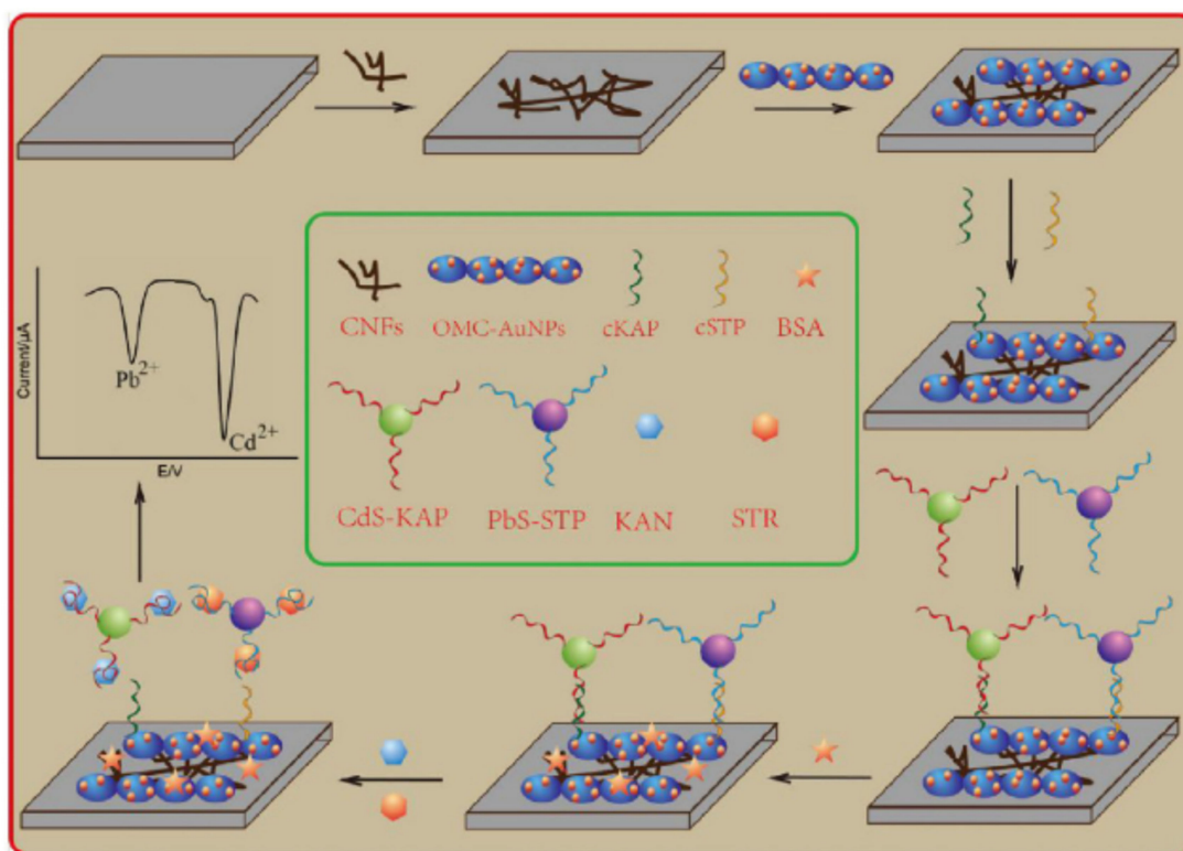
Figure 17. Multiplex electrochemical aptasensor for the multiplex detection of kanamycin and streptomycin in milk based on carbon fiber (CNFs) and mesoporous carbon-gold nanoparticles (OMC-AuNPs). Reprinted from reference [138] with permission from Elsevier.
