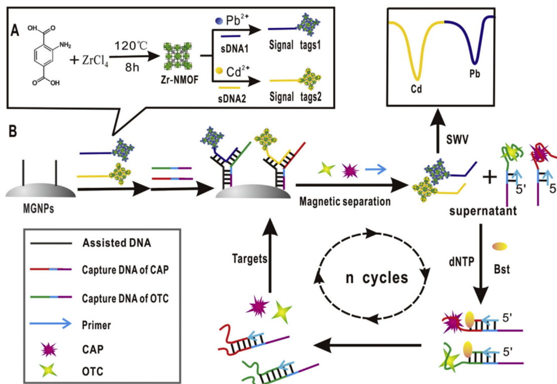
Figure 24. Schematic representation of a multiplex electrochemical aptasensor for the detection of chloramphenicol (CAP) and oxytetracycline (OTC) in milk based on circular strand-replacement DNA polymerization (CSRP). Reprinted from reference [87] with permission from Elsevier.
