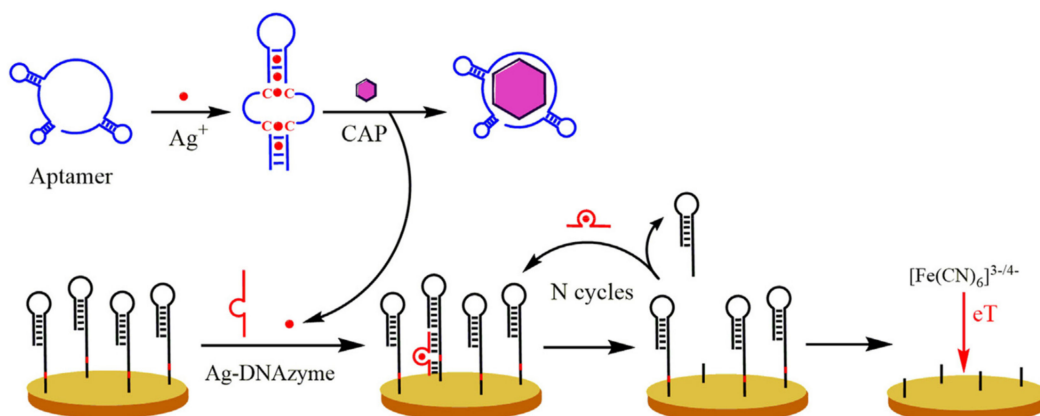
Figure 8. Principle of the aptasensors based on an Ag-DNAzyme for the detection of chloramphenicol (CAP). Reprinted from [37] with permission from Elsevier.
