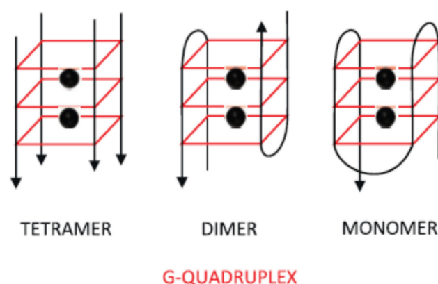
Figure 2. Schematic representation of tetramer, dimer and monomer G-quadruplex structures. The black balls represent the cations that stabilize the structure. Reprinted and adapted from reference [24] with permission from Elsevier.
