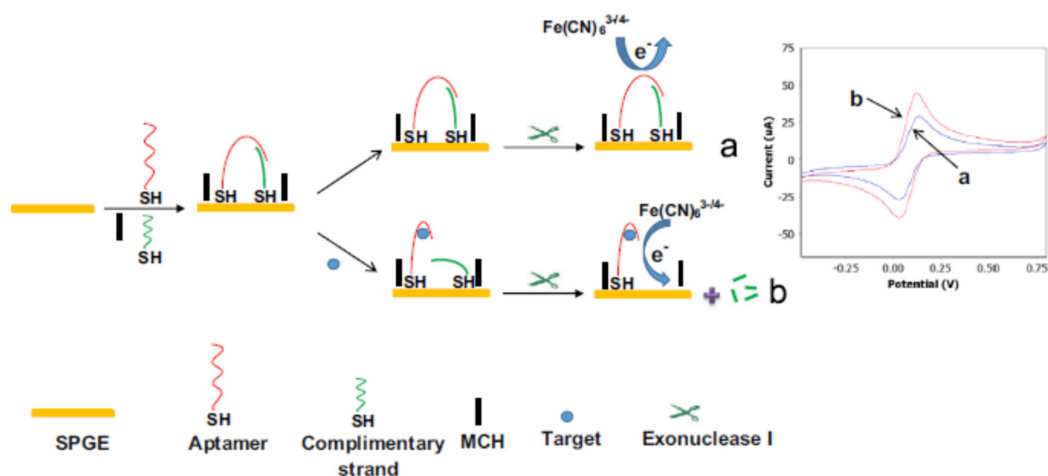
Figure 18. Schematic illustration of the signal amplification by Exonuclease I for the detection of streptomycin in milk. Reprinted from reference [80] with permission from Elsevier.
