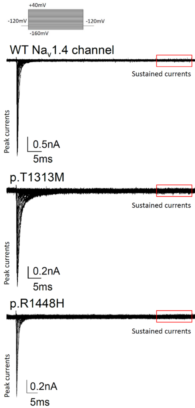
Figure S1. Sample sweeps shows the peak currents and sustained currents in WT, p.T1313M, and p.R1448H mutant Na v 1.4 channels
