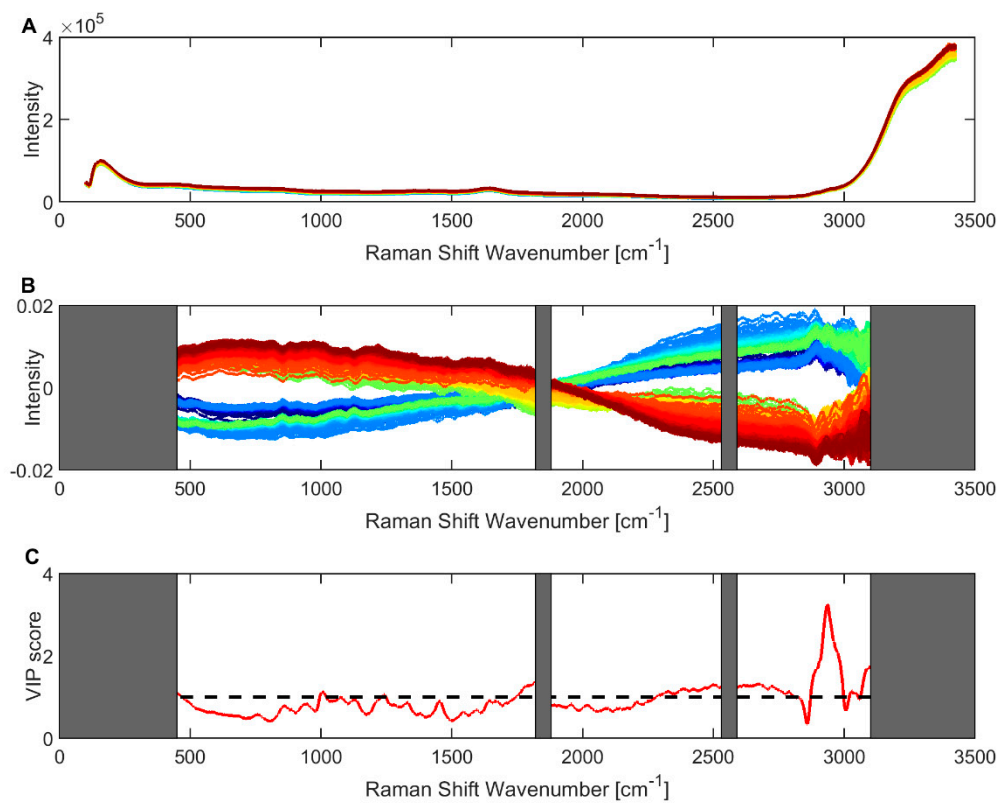
Figure S1. Acquired Raman spectra of the calibration set of ROT1: A contains the raw spectra B shows the pretreated spectra eliminating Raman shift wavenumber regions (100–450 \text{cm}^{-1} , 1820–1880 \text{cm}^{-1} , 2530–2590 \text{cm}^{-1} and 3100–3425 \text{cm}^{-1} ). C contains the Variable Importance in Projection of the calibrated PLS model for ROT1.
