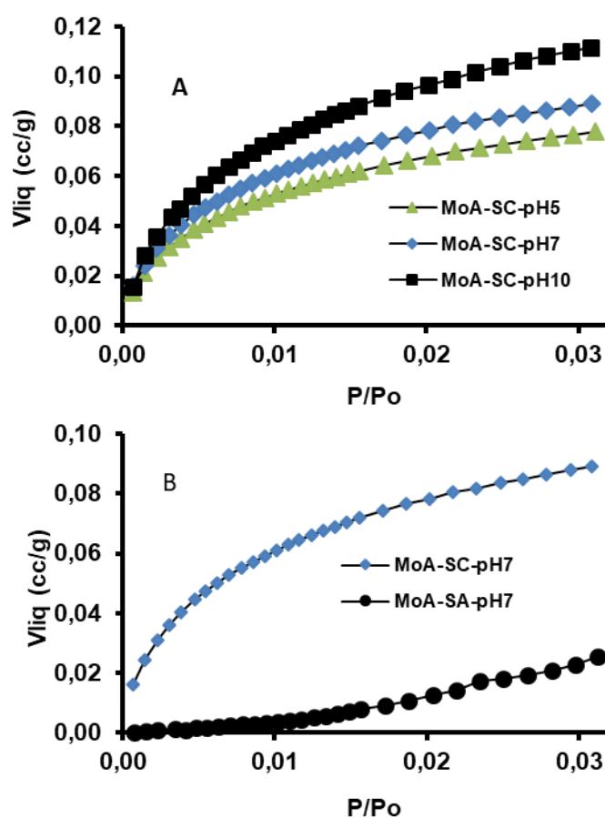
Figure S1. Isotherms of CO 2 -adsorption: (A) Influence of pH and (B) Influence of the surfactant nature.
