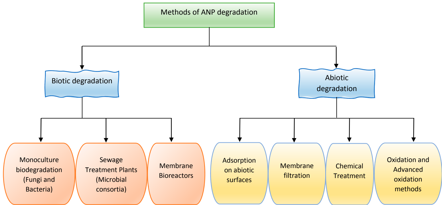
Figure S1: Schematic of existing methods of ANP degradation
