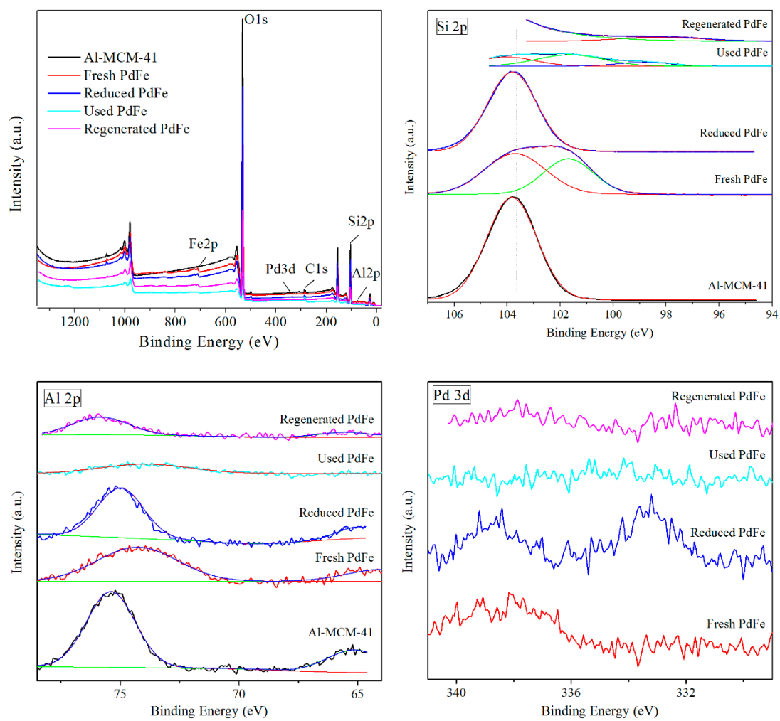
Figure S2. De-convoluted Si 2p, Al 2p and Pd 3d XPS spectra of fresh, used and regenerated Pd-Fe/Al-MCM-41 catalysts.
