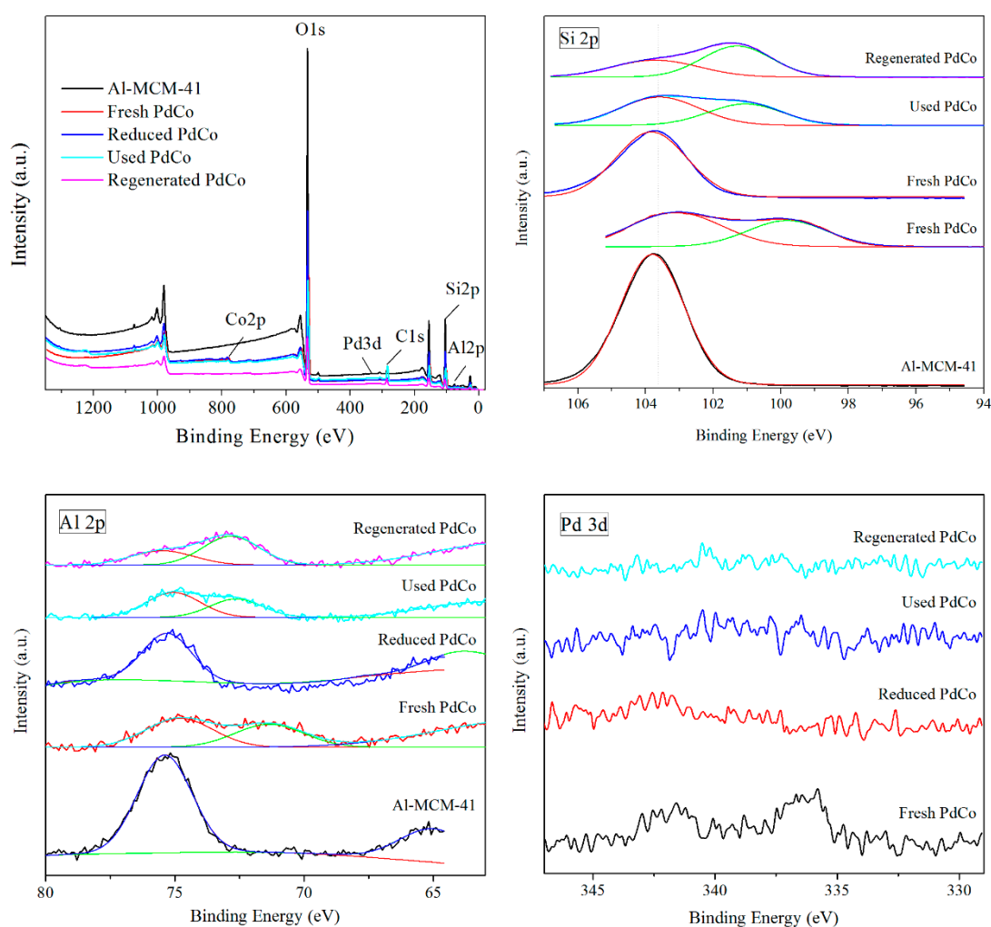
Figure S1. De-convoluted Si 2p, Al 2p and Pd 3d XPS spectra of fresh, used and regenerated Pd-Co/Al-MCM-41 catalysts.
