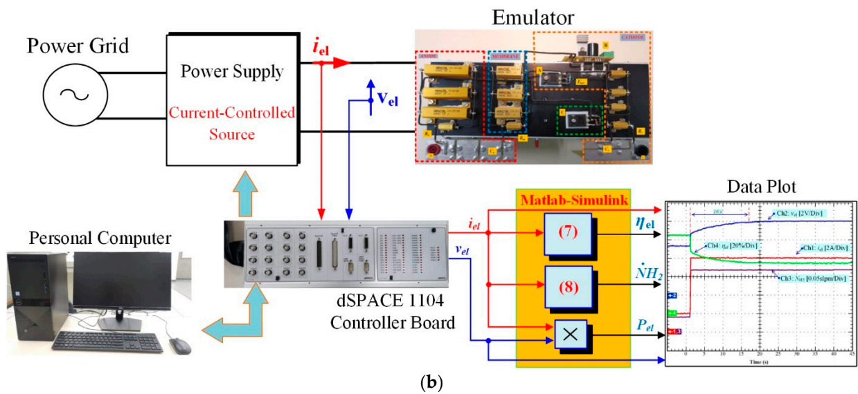
Figure 10. (a). Block diagram of the test rig to acquire data by the electrolyzer. (b). Block diagram of the test rig to test the emulator.
