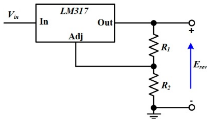
Figure 6. Voltage regulator configuration.
