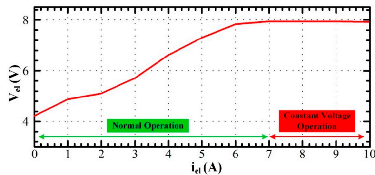
Figure 1. Static voltage-current waveform.
