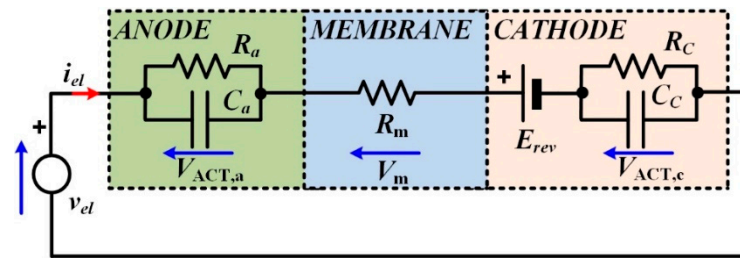
Figure 4. PEM electrolyzer equivalent electrical circuit.
