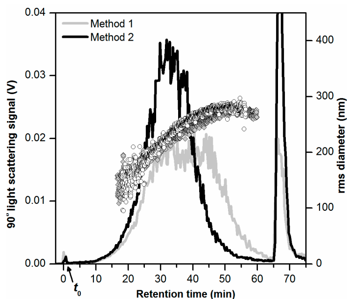
Figure 1. AF4-LS fractograms obtained for toothpaste dispersions (carrier liquid 0.05% w/w SDS, 10 μg injected toothpaste mass) prepared by a two-step dilution in 0.1% w/w SDS (method 1, gray line) and chemical oxidation with 30% H 2 O 2 followed by dilution in 0.1% w/w SDS (method 2, black line). The rms diameter values obtained by MALS are shown as gray diamonds and black circles, respectively. The AF4-LS measurements were performed on different AF4 membranes.
