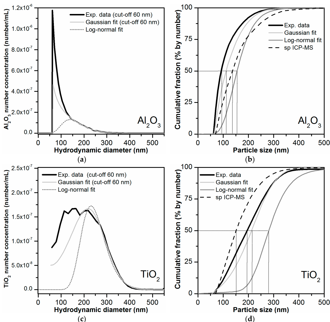
Figure 7. (a,c) Number-based PSDs obtained after mathematical conversion of the mass-based AF4-ICP-MS particle size data. The number-based PSDs obtained after conversion of the original mass-based PSDs (based on the experimental data), and of the fitted curves of the mass-based PSDs (Gaussian and log-normal fits) are shown for comparison. (b,d) Corresponding cumulative PSDs obtained for experimental and the fitted data (Gaussian and log-normal fits). The D50 values obtained for each distribution are highlighted by dotted lines.
