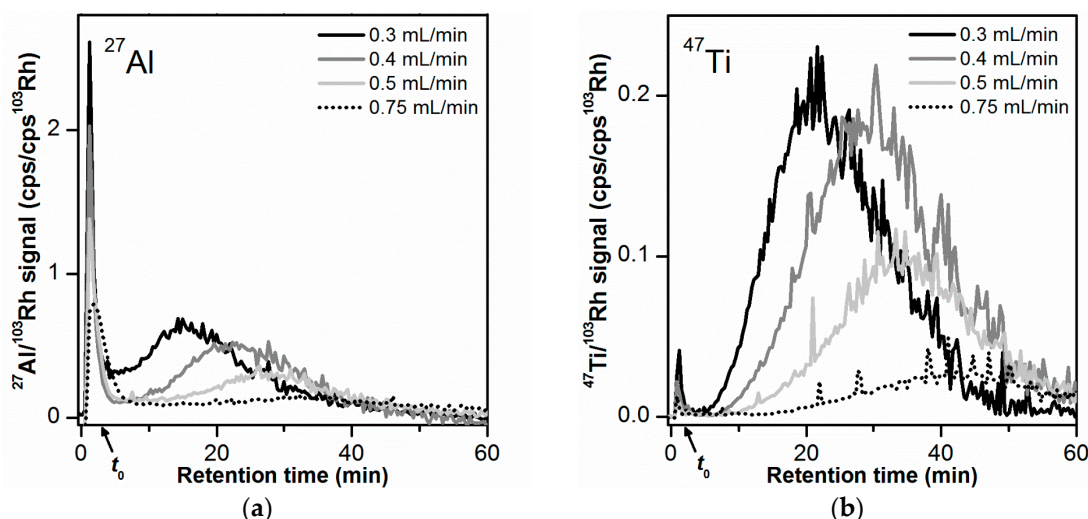
Figure 3. Influence of cross flow rate on the AF4 fractionation of the toothpaste particles (10 µg injected mass): (a) ^{27}\text{Al} signal, (b) ^{47}\text{Ti} signal. All AF4-ICP-MS measurements were performed on the same membrane. Signal smoothing was applied.
