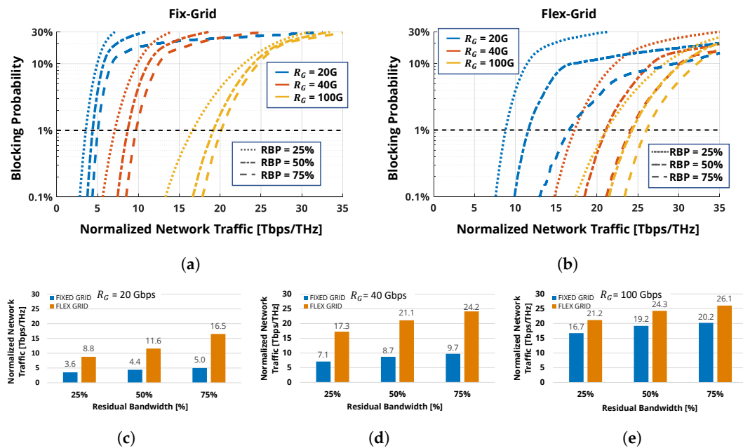
Figure 7. Upper row: blocking probability against the total traffic per residual spectral unit for (a) fix-grid and (b) flex-grid spectral uses. Blue, red and yellow lines refer to R_G of 20, 40, 100 Gbps, respectively. Dotted, dash-dotted and dashed lines refer to 25%, 50% and 75% of residual bandwidth percentage RBP , respectively. Lower row: total traffic per residual spectral unit T at BP_{max} = 1\% for fix- and flex-grid and different RBP for R_G of (c) 20 Gbps; (d) 40 Gbps; (e) 100 Gbps (adapted from [29]).
