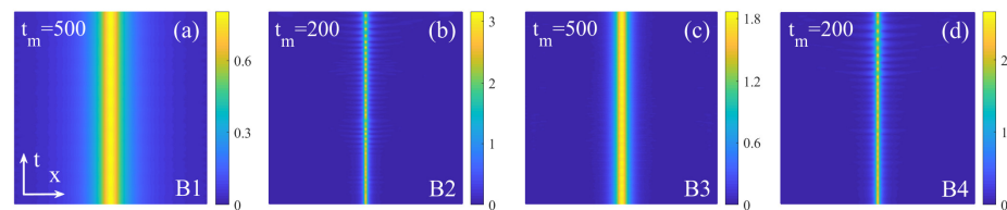
Figure 4. The perturbed evolution of the solitons corresponding to labels B1–B4 in Figure 3a,c. The respective values of the parameters are \alpha = 1.1 , g = 1 , \mu = -0.2 (a); \alpha = 1.1 , \mu = -2 (b); \alpha = 1.7 , \mu = -1.5 (c); \alpha = 1.1 , \mu = -1.5 (d). The evolution is plotted in the spatial domain -10 < x < +10 . Values t_m indicate intervals of the scaled propagation distance in the respective panels, 0 < z < t_m . In panels (a,c), larger t_m is taken to corroborate the full stability of the solitons. The plots are borrowed from Reference [47] (unpublished).
