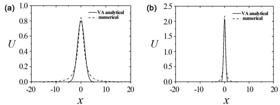
Figure 1. Profiles of solitons with \mu = -0.3 (a) and -2.0 (b), predicted by the VA based on the Gaussian ansatz (23) and Euler–Lagrange equations (26) and their counterparts produced by the numerical solution of Equation (8) with Lévy index \alpha = 1.5 and g = 1 . Reprinted with permission from Reference [39]. Copyright 2020 Elsevier.
