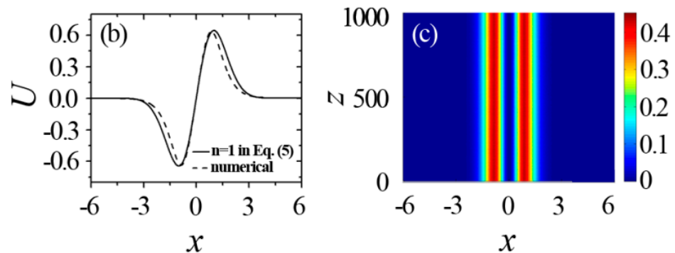
Figure 5. An example of a stable dipole-mode soliton produced by Equation (1) with Lévy index \alpha = 1 , parabolic trapping potential (32) with \Omega^2 = 1 , i.e., V(x) = 0.5x^2 , and nonlinearity strength g = 0.5 . The propagation constant of this state is -\mu = 1.16 . The stationary profiles of the soliton and its propagation, in terms of the local-power distribution, are displayed in the left and right panels, respectively. The solid line in the left panel represents the analytical fit provided by Equation (33) with n = 1 . Adapted with permission from Reference [34]. Copyright 2020 Elsevier. Panel (a) from the original figure is not included here, as it is not necessary.
