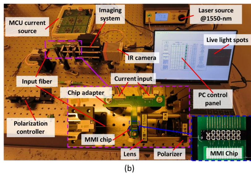
Figure 3. (a) Diagram and (b) actual photo of the FPWE system.
