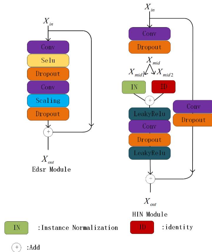
Figure 5. Structure of Edsr Module and HIN Module.
