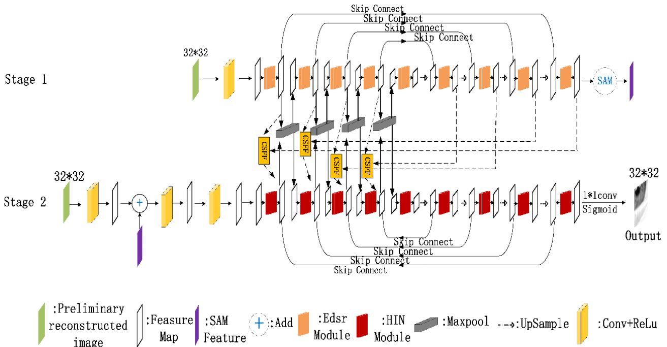
Figure 4. Structure of the DIP reconstruction network.
