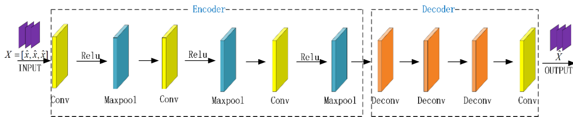
Figure 6. The structure of the denoising autoencoder.
