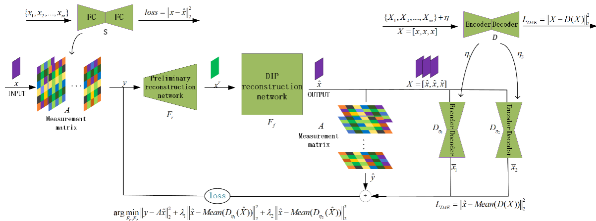
Figure 3. Structure of the proposed DPAP, where Mean(\cdot) means to average the three-channel image.
