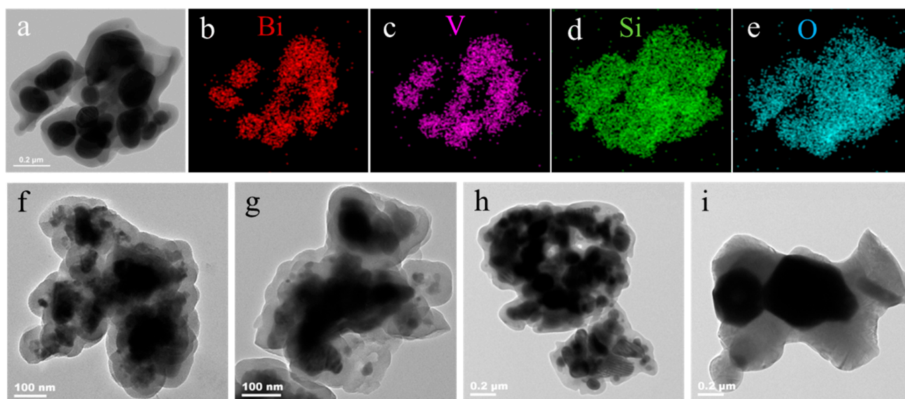
Figure 4. (a) TEM image and (b–e) corresponding EDS elemental mapping of \text{BiVO}_4@\text{SiO}_2 with 20 g of TEOS added and calcination at 500 °C. TEM images of \text{BiVO}_4@\text{SiO}_2 at different calcination temperatures of (f) 500 °C, (g) 600 °C, (h) 700 °C, and (i) 800 °C.
