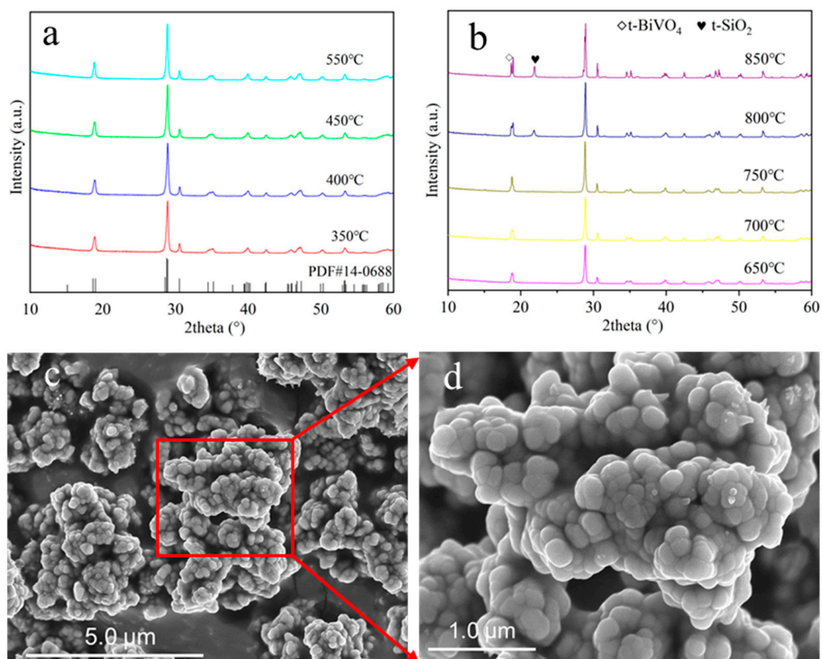
Figure 3. XRD patterns of \text{BiVO}_4@\text{SiO}_2 (a,b) calcined at different temperatures for 6 h. (c) SEM images of \text{BiVO}_4@\text{SiO}_2 encapsulated pigment calcined at 500 °C and (d) corresponding enlarged view of the selected area.
