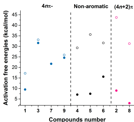
Figure 10. Activation free energies (kcal/mol) of all compounds 1–9 at the (U)B3LYP/6-311G(d,p) level in the S 0 (unfilled circles) and T 1 (filled circles) states.
