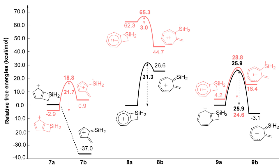
Figure 9. Free energy changes in 5- and 7-membered annulenyl cations and anions fused with SCB rings upon ring-openings at (U)B3LYP/6-311G(d,p) level. Compound 7a ( S_0 ) is not a minimum in the S_0 state. The black energy levels represent S_0 and those of red indicate T_1 state and energies for transition states are given in bold.
