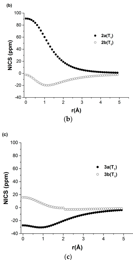
Figure 6. Nucleus independent chemical shifts (NICS) scans of (a) 1a(T_1) and 1b(T_1) ; (b) 2a(T_1) and 2b(T_1) ; as well as (c) 3a(T_1) and 3b(T_1) at the GIAO-(U)B3LYP/6-311+G(d,p)//(U)B3LYP/6-311G(d,p) level. Only the out-of-plane components are displayed.
