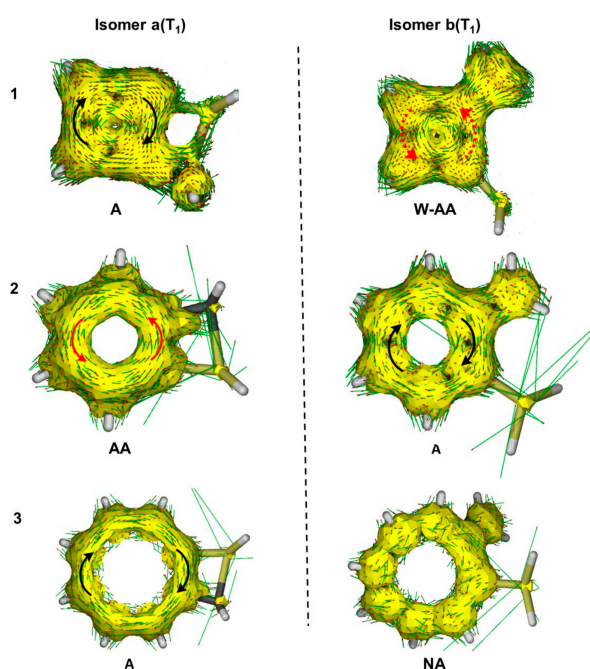
Figure 7. Anisotropy of the induced current density (ACID) plots at (U)B3LYP/6-311+G(d,p)//(U)B3LYP/6-311G(d,p) level. Broken arrows in 1b(T_1) indicate weaker ring-currents. Aromatic = A, antiaromatic = AA, weakly antiaromatic = WAA, and non-aromatic = NA.
