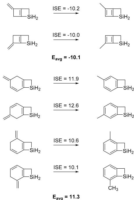
Figure 8. Isomerization stabilization energy (ISE) values (kcal/mol) of the 4- and 5-methyl substituted 1a(T_1) derivatives, and the 5-, 6-, 7-, and 8-methyl substituted 2a(T_1) derivatives at the UB3LYP/6-311G(d,p) level. ISE_{\text{avg}} is the average ISE value for the various methyl substitutions.
