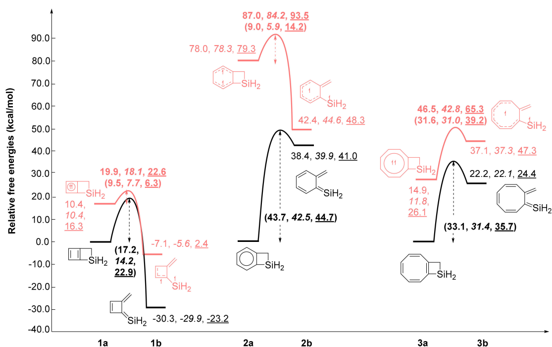
Figure 3. T_1 state potential free energy surface diagrams for ring-openings of 2,3-cyclobutadieno-1-SCB ( 1 ), 2,3-benzo-1-SCB ( 2 ) and 2,3-cyclooctatetraeno-1-SCB ( 3 ) at (U)B3LYP/6-311G(d,p) (normal print), (U)OLYP/6-311G(d,p) (italics), and (U)CCSD(T)/6-311G(d,p)/(U)B3LYP/6-311G(d,p) (underlined) levels. Values in parenthesis are activation energies. Values for the S_0 state in black and values for the T_1 state in red.
