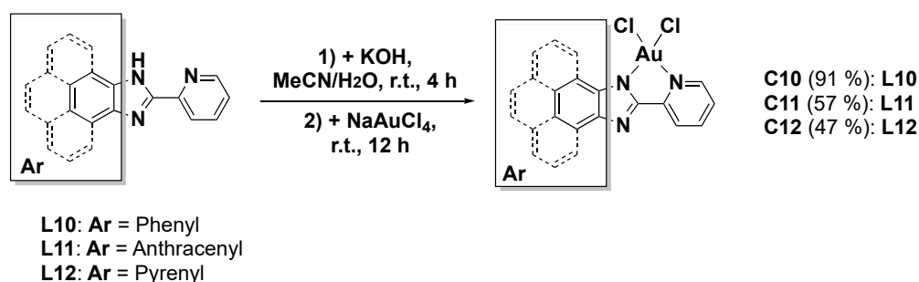
Scheme 1. Synthetic pathways to the series of cationic (top) and neutral (bottom) Au(III) complexes C1–C9 and C10–C12 , respectively.
