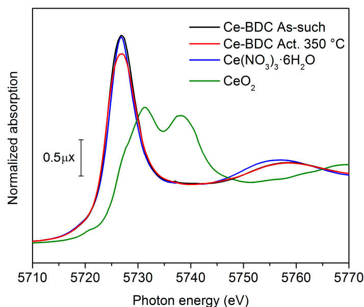
Figure 3. Ce L 3 edge XANES spectra of Ce 5 (BDC) 7.5 (DMF) 4 as synthesized and activated at 350 °C, compared with CeO 2 and Ce(NO 3 ) 3 ·6H 2 O.
