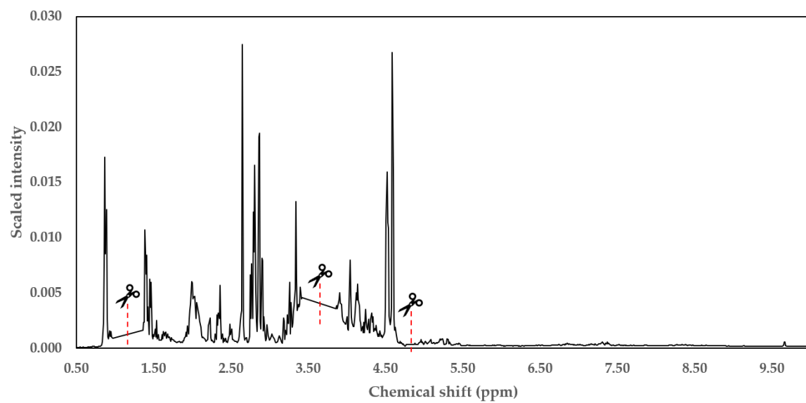
Figure S2. Representative ^1\text{H} NMR spectrum of a wine sample (after preprocessing)
