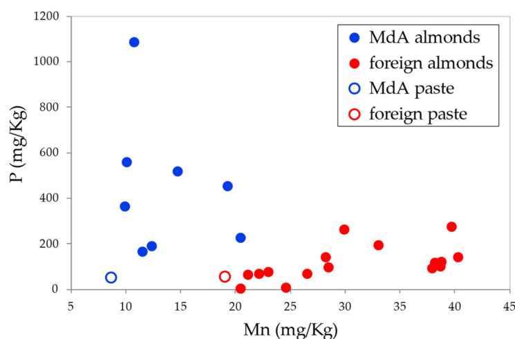
Figure 4. Biplot Mn vs. P.
