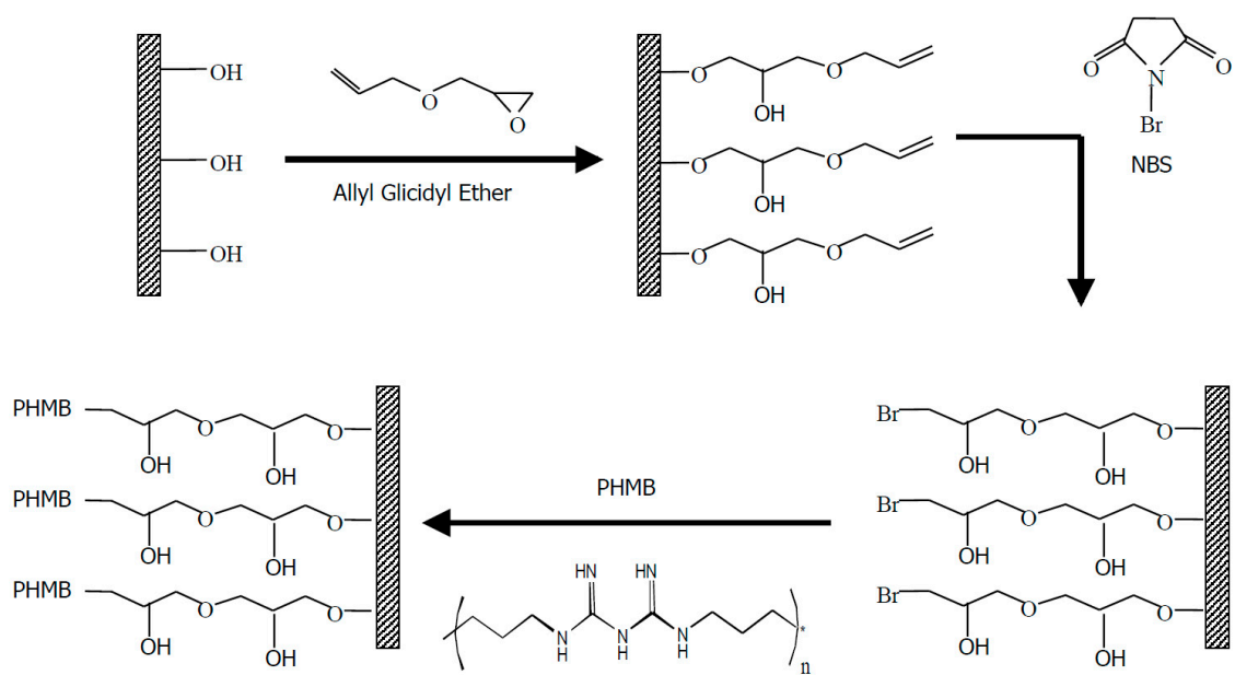
Figure S1. Structures for immobilization chemistry.
