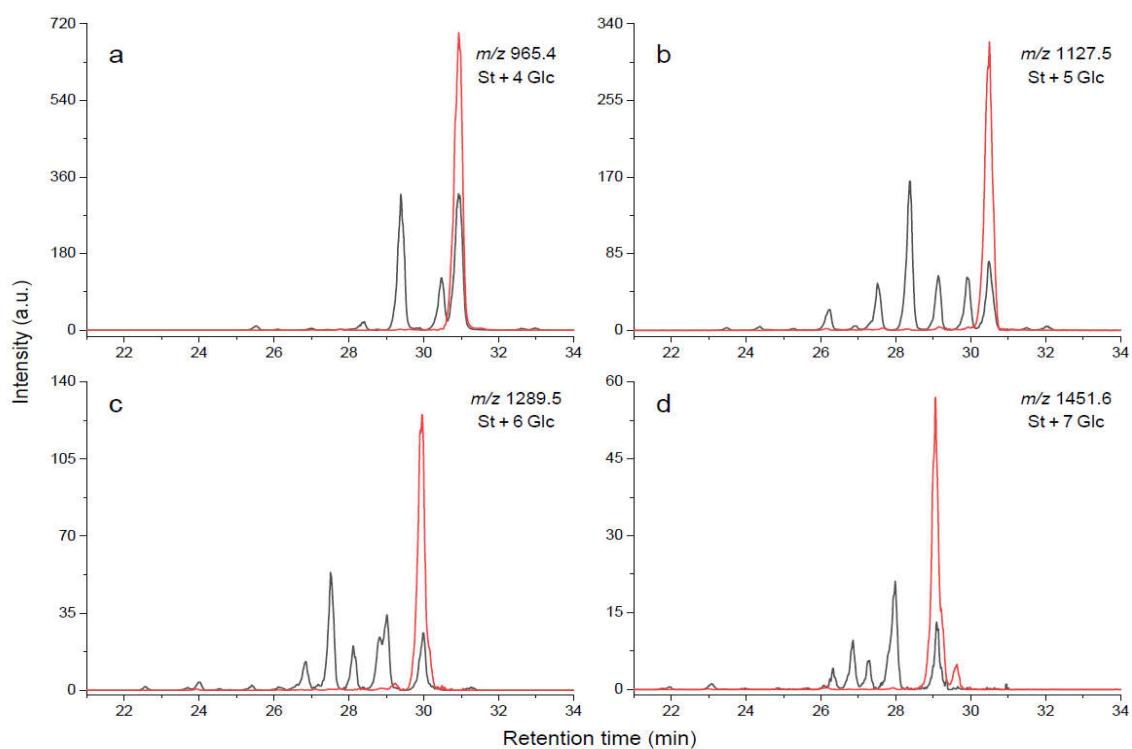
Figure 1. Extracted ion chromatograms for glucosylated products of SVglys (black line) and RebA (red line) corresponding to m/z 965.4 (a), 1127.5 (b), 1289.5 (c) and 1451.6 (d).
