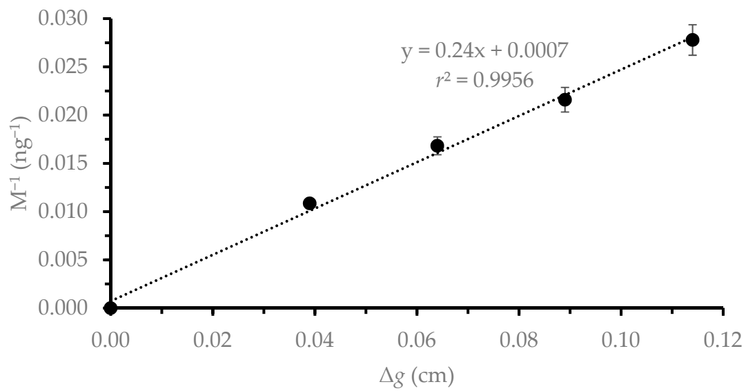
Figure S1. Measured mass of mercury in the binding gels immersed in Hg model solution for different thicknesses of diffusive gel.
