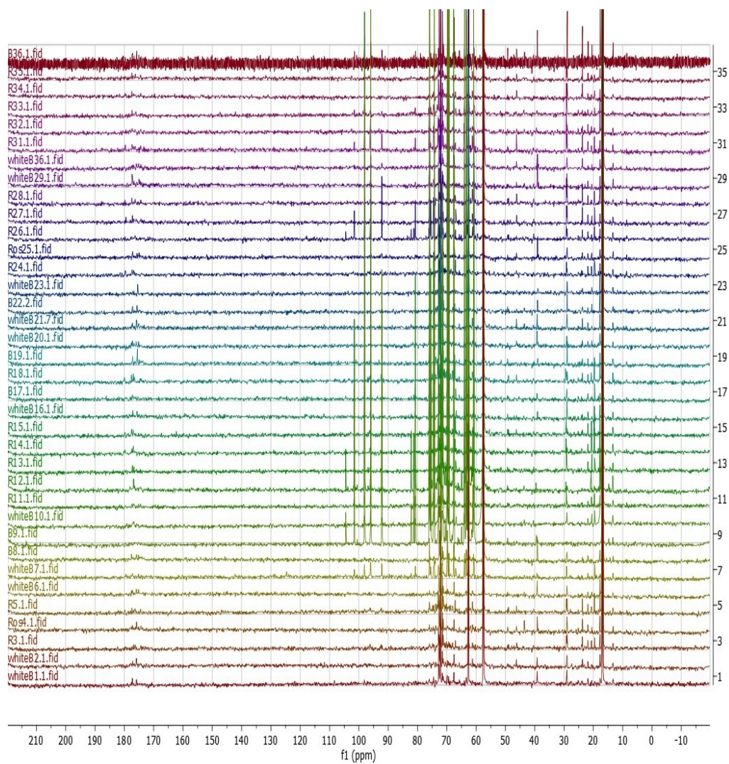
Supplementary Figure 1. ^{13}\text{C} - ^1\text{H} NMR spectra recorded during the analysis of wine samples of different varieties.
