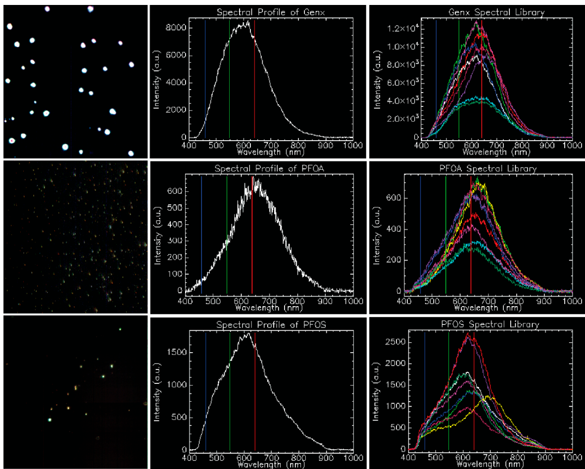
Figure S1. Hyperspectral images and spectral profiling of GenX (top row), PFOA (middle row) and PFOS (bottom row).
