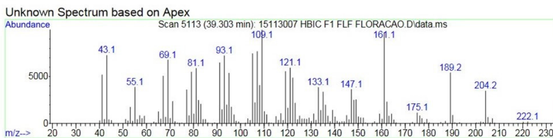
Figure S2. Mass spectrum of Non-identified compound 2 (N.I. 2) detected in the essential oil of H. brasiliense from Ilha do Cardoso.
