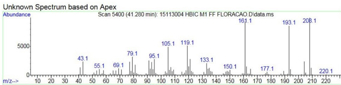
Figure S4. Mass spectrum of Non-identified compound 4 (N.I. 4) detected in the essential oil of H. brasiliense from Ilha do Cardoso.
