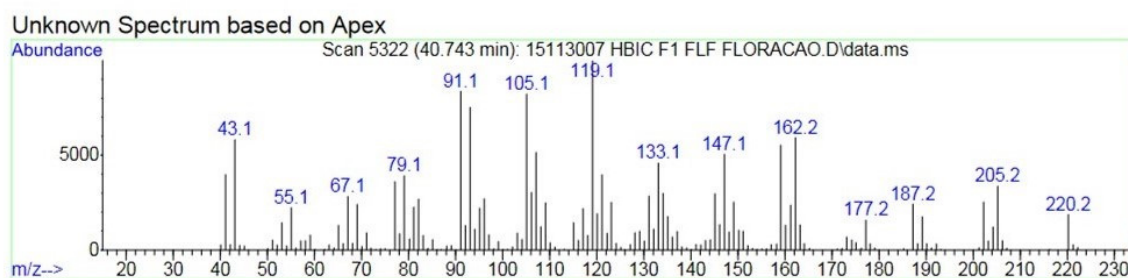
Figure S3. Mass spectrum of Non-identified compound 3 (N.I. 3) detected in the essential oil of H. brasiliense from Ilha do Cardoso.
