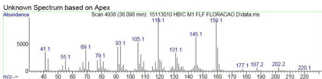
Figure S1. Mass spectrum of Non-identified compound 1 (N.I. 1) detected in the essential oil of H. brasiliense from Ilha do Cardoso.
