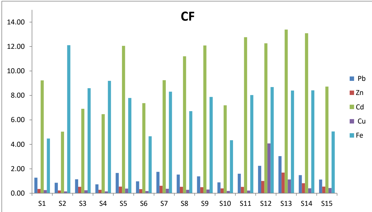
Contamination Factor of Surface Sediment in Perak River
