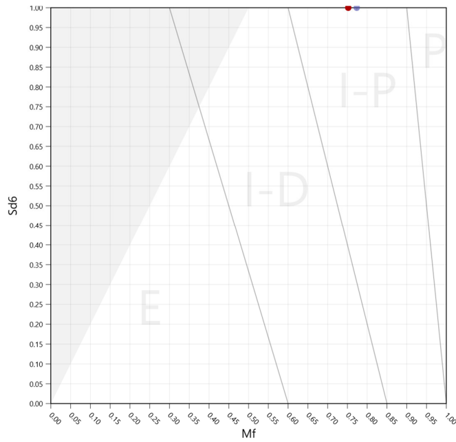
Figure S2. Temporary Regime Plot (TRP) of Tsiknias river in natural (red) and actual conditions (blue).
