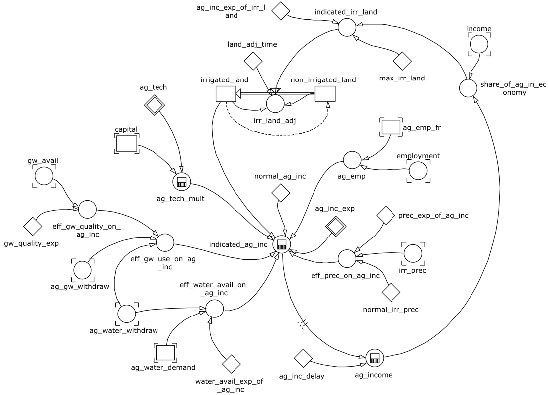
Figure 3.1: Causal structure of the agriculture production module
