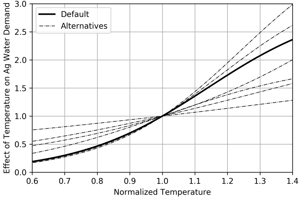
Figure 2.4: Effect of temperature on ag water demand (Equation 2.18)
