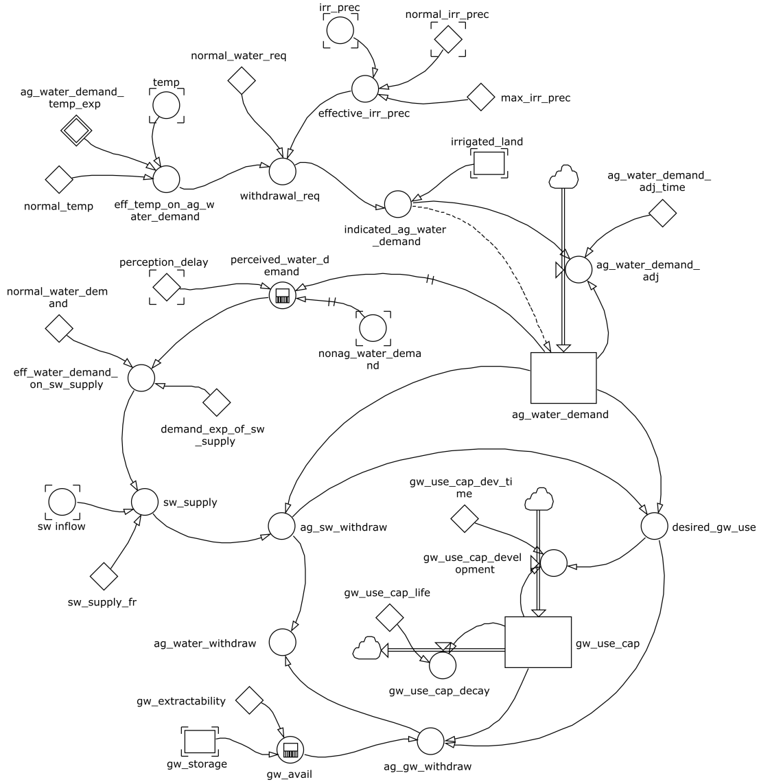
Figure 2.2: Causal structure of the agriculture water use module
