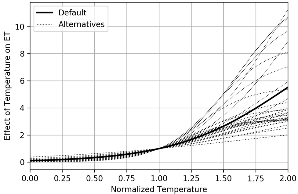
Figure 1.6: Effect of temperature on evapotranspiration (Equation 1.39)
