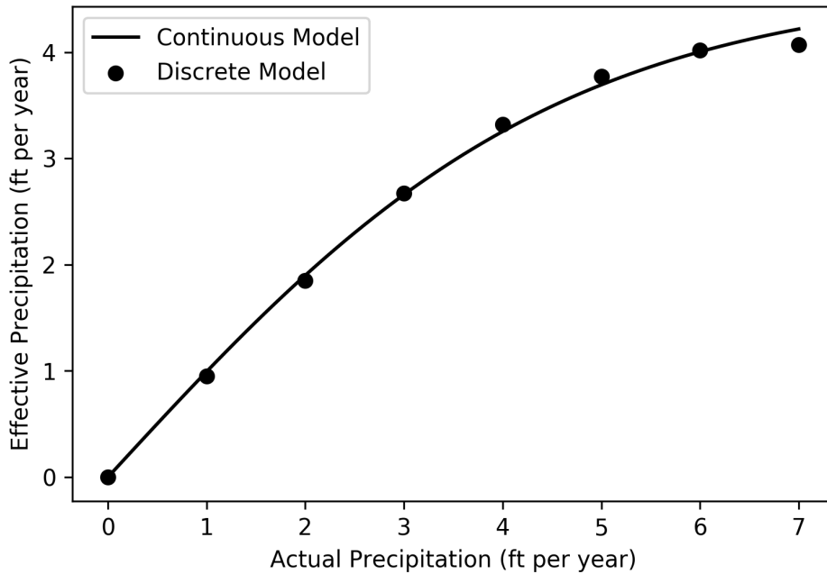
Figure 2.5: Continuous vs discrete model for prediction of effective precipitation (Equation 2.20)
