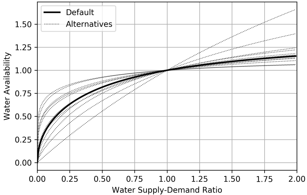
Figure 2.9: Water availability index (Equation 2.48)
