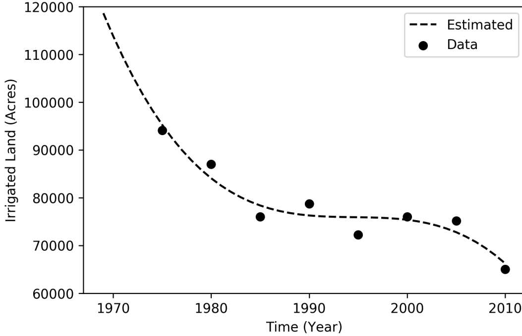
Figure 3.3: Trend of irrigated land in the lower Rio Grande region
