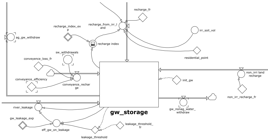
Figure 1.9: Causal structure of the hydrology module – groundwater
