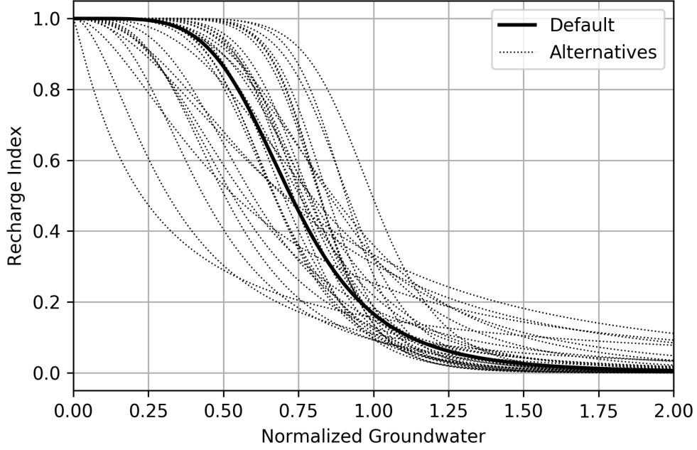
Figure 1.7: Recharge index as a function of groundwater level (Equation 1.44)
