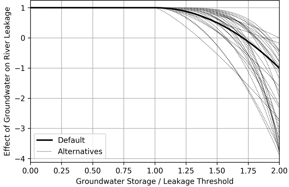
Figure 1.3: Effect of groundwater level on the river leakage rate (Equation 1.14)
