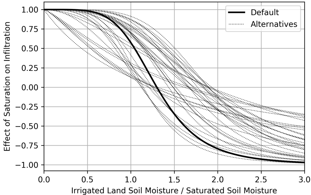
Figure 1.4: Effect of soil moisture saturation on infiltration rate (Equation 1.22)
