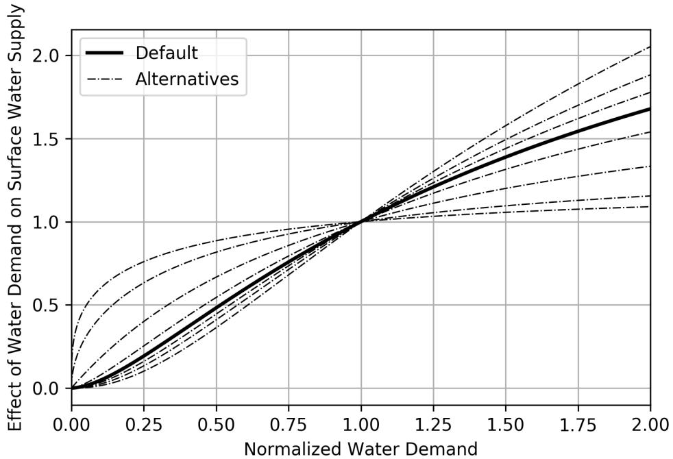
Figure 2.6: Effect of water demand pressure on surface water supply (Equation 2.26)
