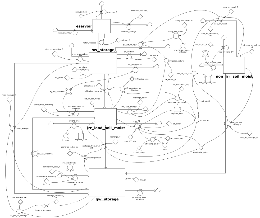
Figure 1.1: Causal structure of the hydrology module
