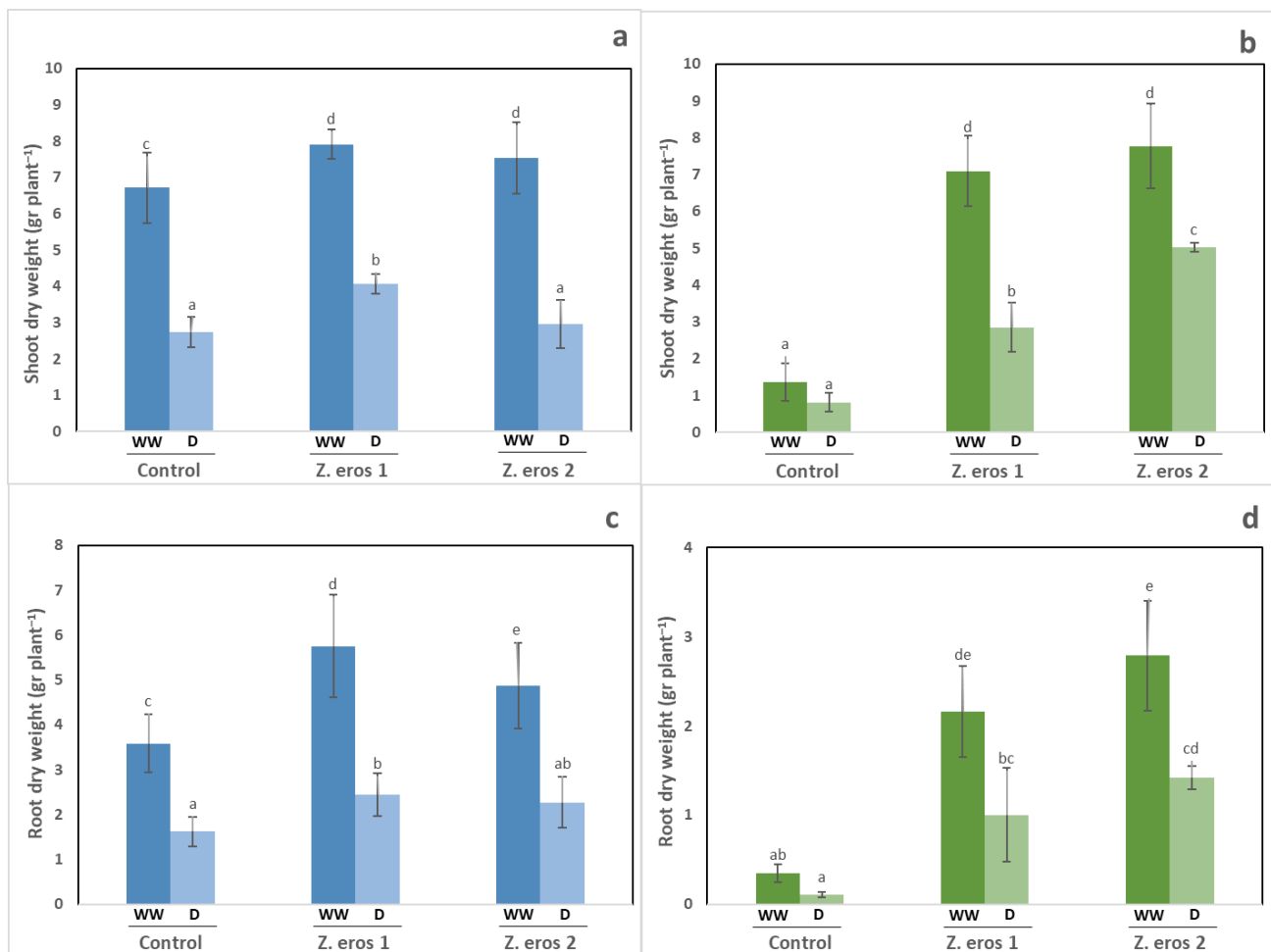
Figure 1. Shoot and root dry weight of wheat plants (a,c) and tomato plants (b,d) inoculated with the fungal endophytes Z. erostrata 1 y Z. erostrata 2 and cultivated under well-watered (WW) and drought stress (D) conditions. The data are the means \pm standard deviation of ten replicates. Different letters indicate significant differences between all treatments, according to Duncan's multiple-range test ( p < 0.05 ).
