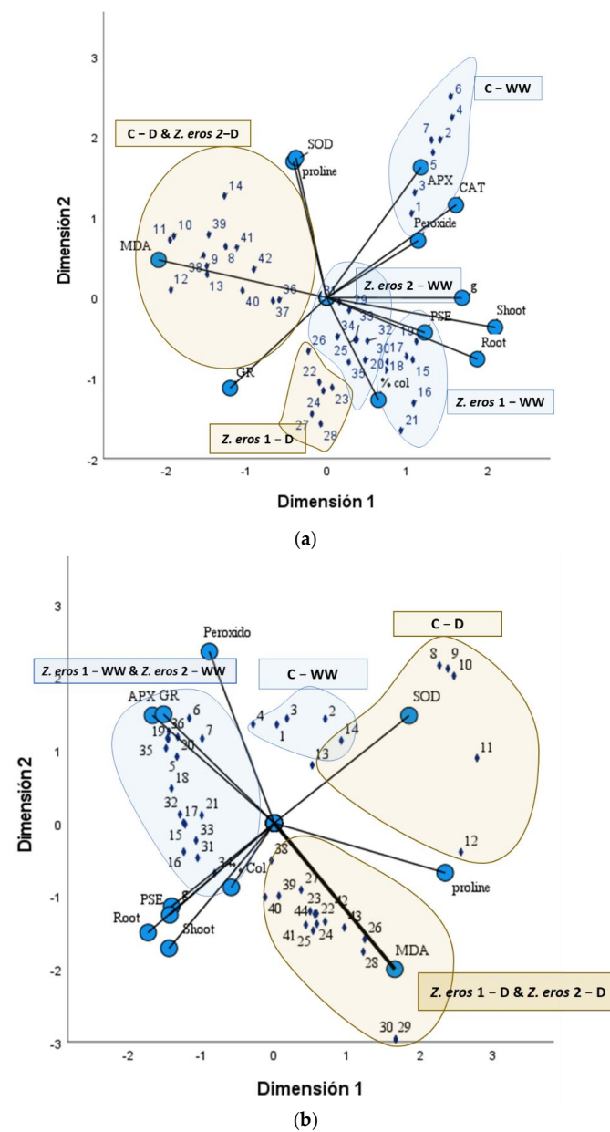
Figure 6. Categorical Principal Component Analysis (CATPCA) of wheat (a) and tomato (b) plant samples (indicated by dark blue diamonds) measured through antioxidant enzyme activities (SOD,
