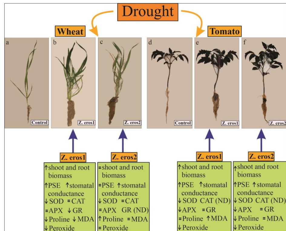
Figure 7. Effects triggered by two endophytic fungal strains ( Z. erostrata 1 and Z. erostrata 2) to alleviate drought in wheat and tomato plants. Wheat plants (a–c) and tomato plants (d–f), uninoculated controls and plants inoculated with the fungal endophytes Z. erostrata 1 y Z. erostrata 2 subjected to drought stress conditions. ↑ arrows show an increase, while ↓ arrows show a decrease in the variable. The sign = indicates no significant changes in the parameter, and ND: indicates not detected.
