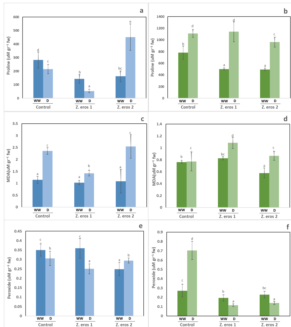
Figure 5. Proline content (a,b), MDA (c,d) and hydrogen peroxide content (e,f) in wheat and tomato plants respectively. Plants were inoculated with the fungal endophytes Z. erostrata 1 y Z. erostrata 2 and cultivated under well-watered (WW) or drought (D) conditions. Values are the means \pm standard deviation of four replications. According to Duncan's multiple-range test ( p < 0.05 ), different letters indicate significant differences between all treatments.
