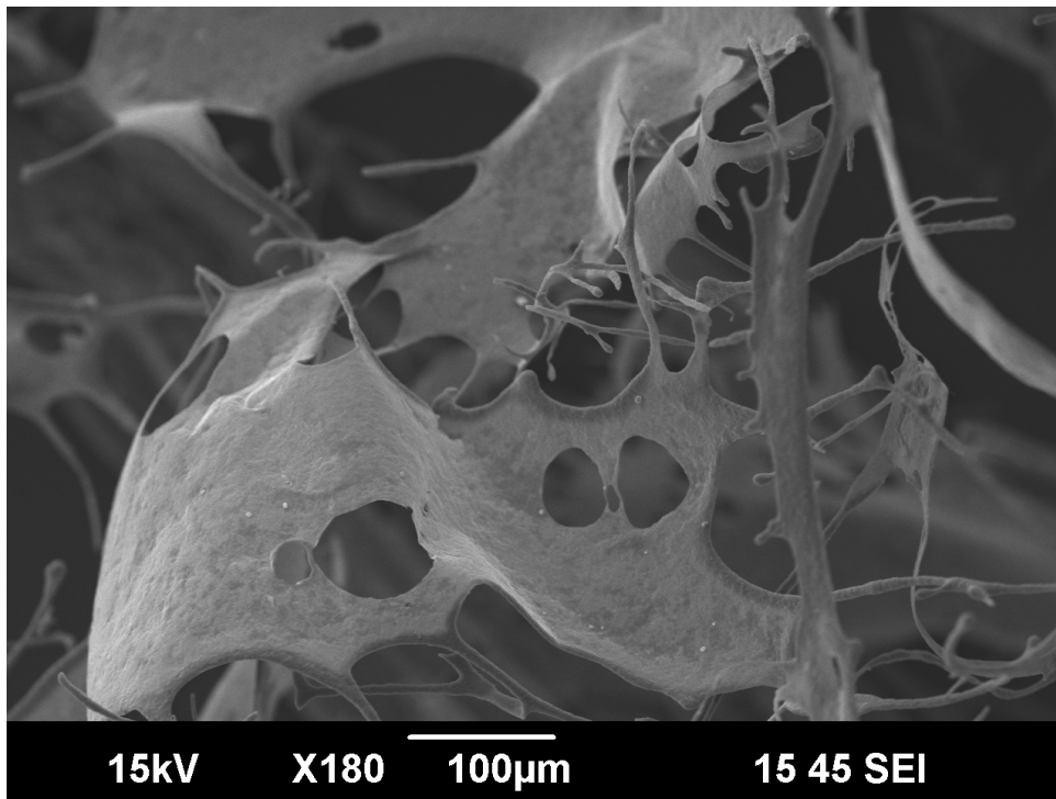
Figure S1: SEM micrograph of cross-linked cryogel of composite A.
