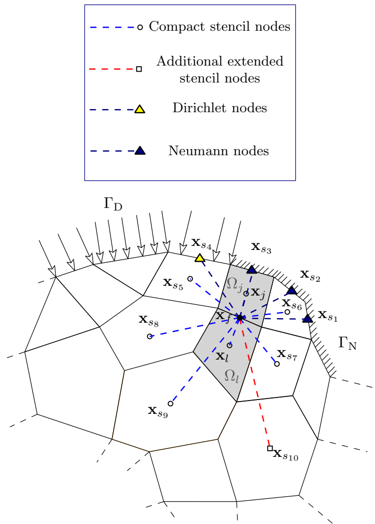
Figure 5. Face stencils with boundary nodes.
