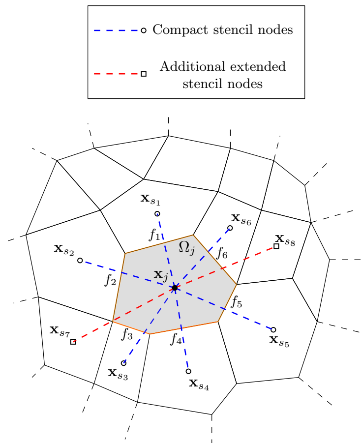
Figure 3. Compact and extended cell stencils.
