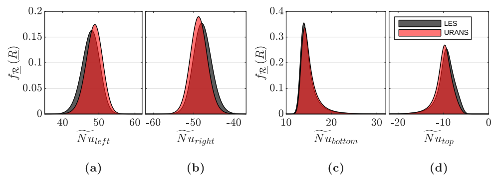
Figure 13. Probability density functions for the integral mean Nusselt number: (a) on the left wall, \widetilde{Nu}_{left} ; (b) on the right wall, \widetilde{Nu}_{right} ; (c) on the bottom wall, \widetilde{Nu}_{bottom} ; and (d) on the top wall, \widetilde{Nu}_{top} .
