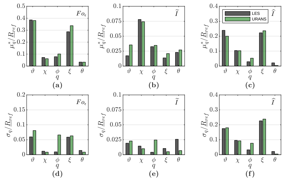
Figure 12. Normalized modified mean \mu_q^*/\underline{\mathbf{R}}_{ref} and standard deviation \sigma_q/\underline{\mathbf{R}}_{ref} for the responses: (a,d) for the mixing time Fo_\epsilon , (b,e) for the integral mean segregation intensity \tilde{I} , and (c,f) for the mean absolute deviation to the reference case of the segregation intensity \hat{I} .
