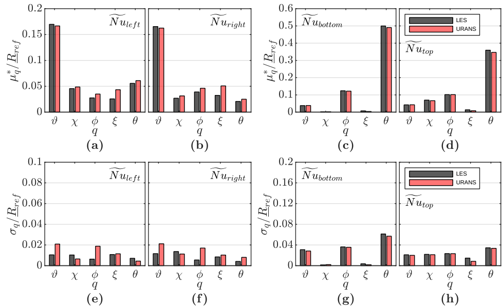
Figure 9. Normalized modified mean \mu_{q_i}^*/\mathbf{R}_{ref} and standard deviation \sigma_{q_i}/\mathbf{R}_{ref} of the integral mean Nusselt number: (a,e) on the left wall, \widetilde{N}u_{left} ; (b,f) on the right wall, \widetilde{N}u_{right} ; (c,g) on the bottom wall, \widetilde{N}u_{bottom} ; and (d,h) on the top wall, \widetilde{N}u_{top} .
