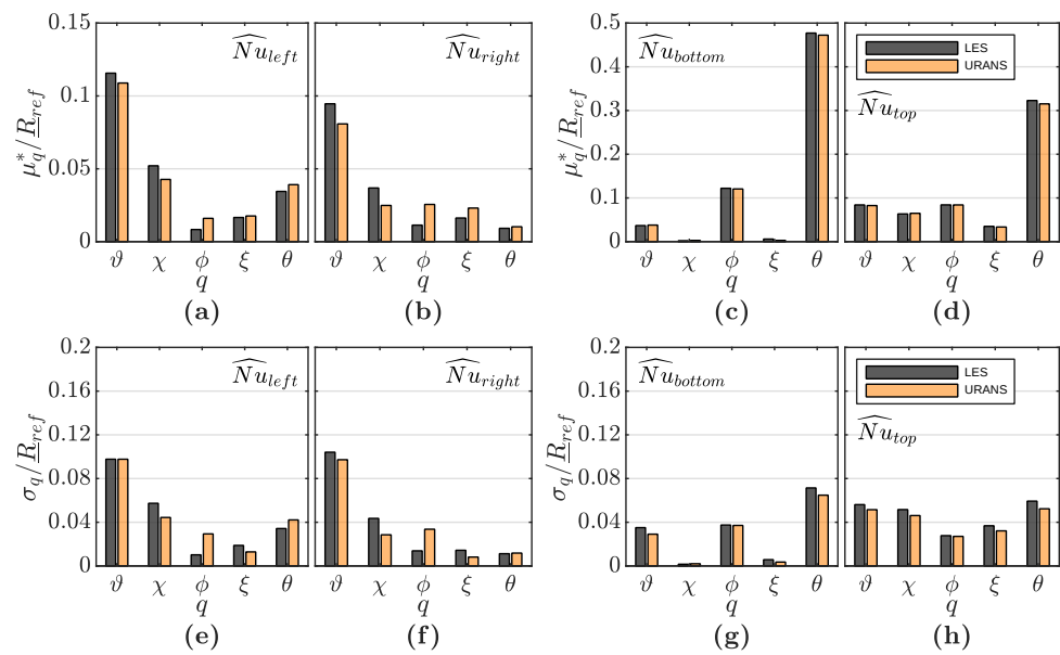
Figure 10. Normalized modified mean \mu_q^*/\mathbf{R}_{ref} and standard deviation \sigma_q/\mathbf{R}_{ref} of the mean absolute deviation to the reference case of the Nusselt number: (a,e) on the left wall, \widehat{Nu}_{left} ; (b,f) on the right wall, \widehat{Nu}_{right} ; (c,g) on the bottom wall, \widehat{Nu}_{bottom} ; and (d,h) on the top wall, \widehat{Nu}_{top} .
