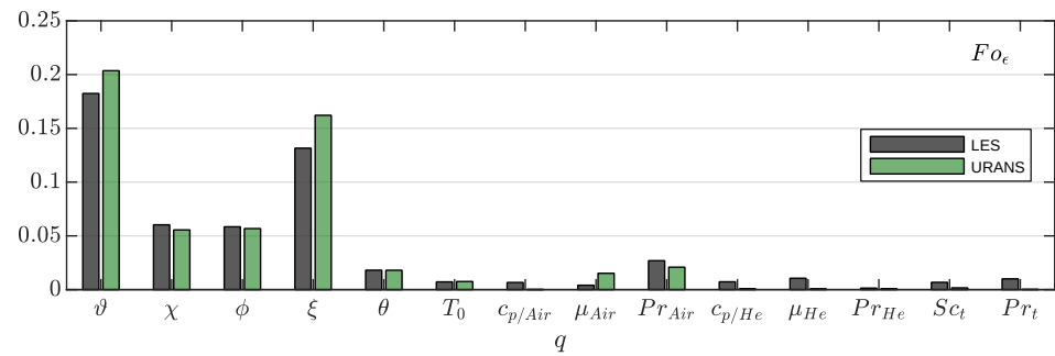
Figure 8. Normalized modified mean \mu_q^*/\mathbf{R}_{ref} for the mixing time Fo_\epsilon for LES and URANS.
