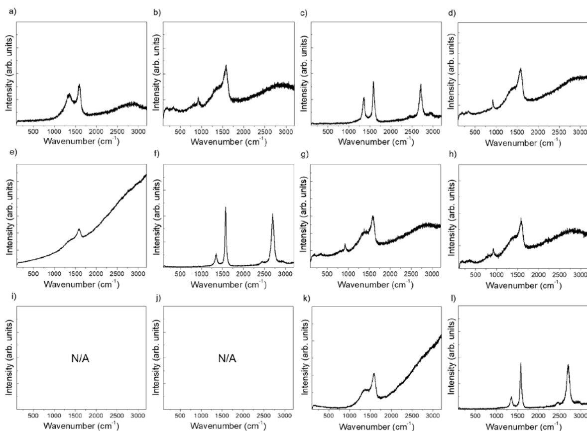
Figure S1. The Raman spectra (514.5 nm) for CNT samples grown using FeMoC as a catalyst.
