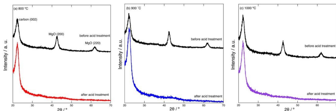
Figure 1. XRD patterns of the carbonized products prepared by heating at (a) 800 °C, (b) 900 °C, and (c) 1000 °C: Before sulfuric acid treatment (black) and after sulfuric acid treatment (red, blue, and purple).
