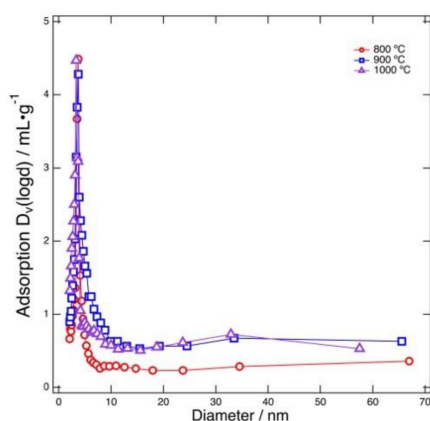
Figure 5. Pore size distributions of carbonized products.
