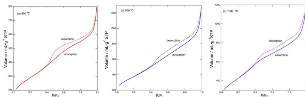
Figure 4. Adsorption and desorption isotherms of the carbonized products prepared by heating at (a) 800 °C, (b) 900 °C, and (c) 1000 °C.
