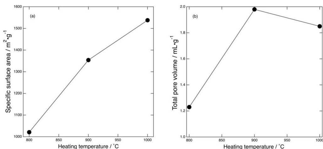
Figure 6. Specific surface area (a) and total pore volume (b) as a function of heating temperature.
